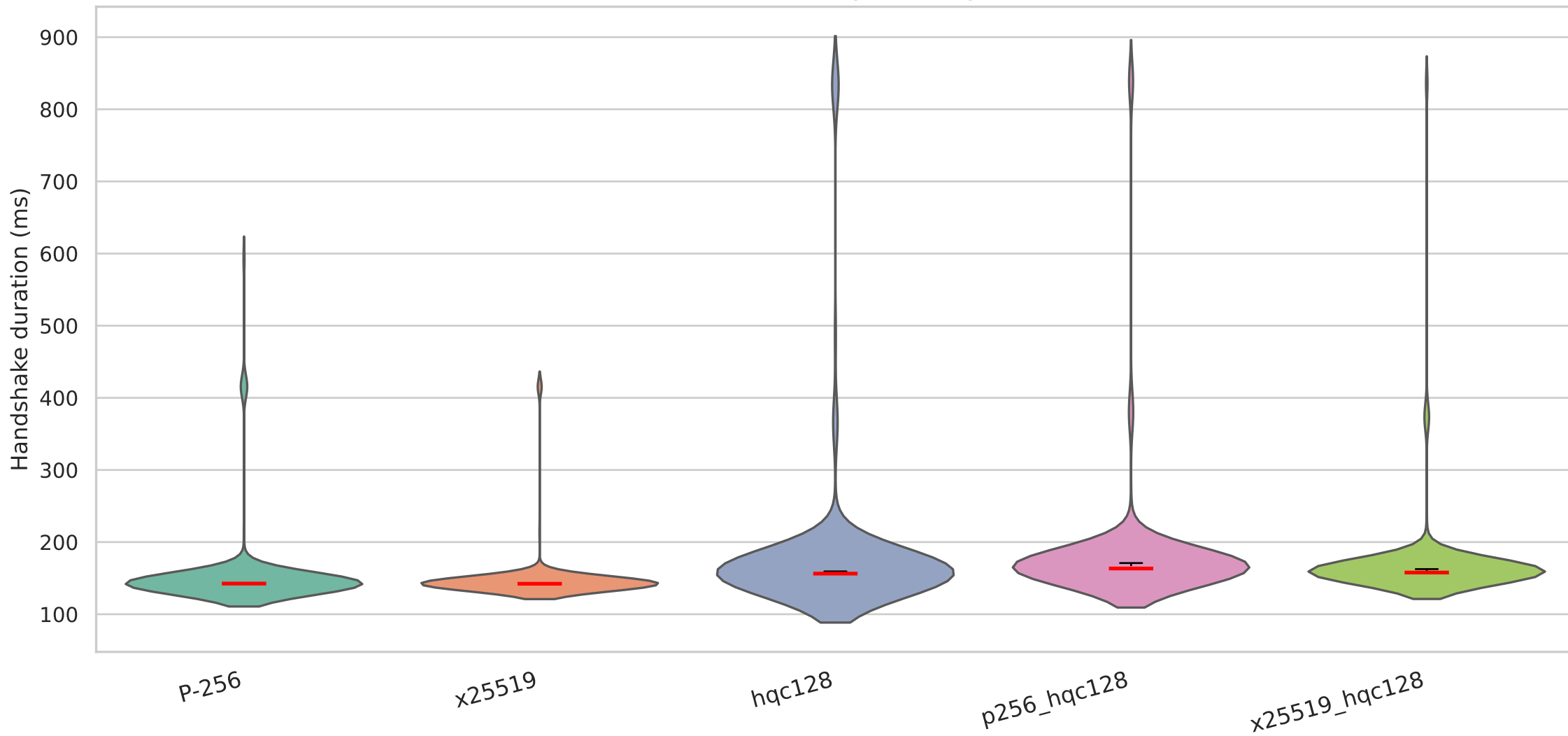
Handshake duration on QUIC with mldsa44 signature algorithm — Local YDE (35ms/2%)
