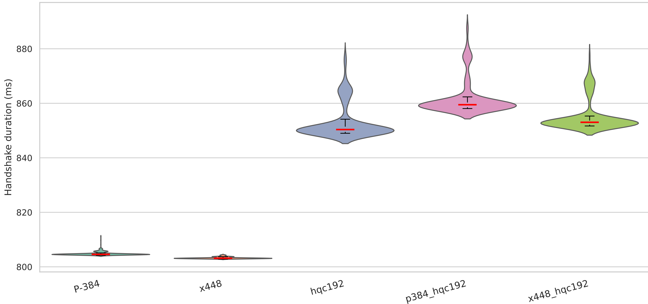
Handshake duration on QUIC with mlds65 signature algorithm — Backbone (200ms/4%)
