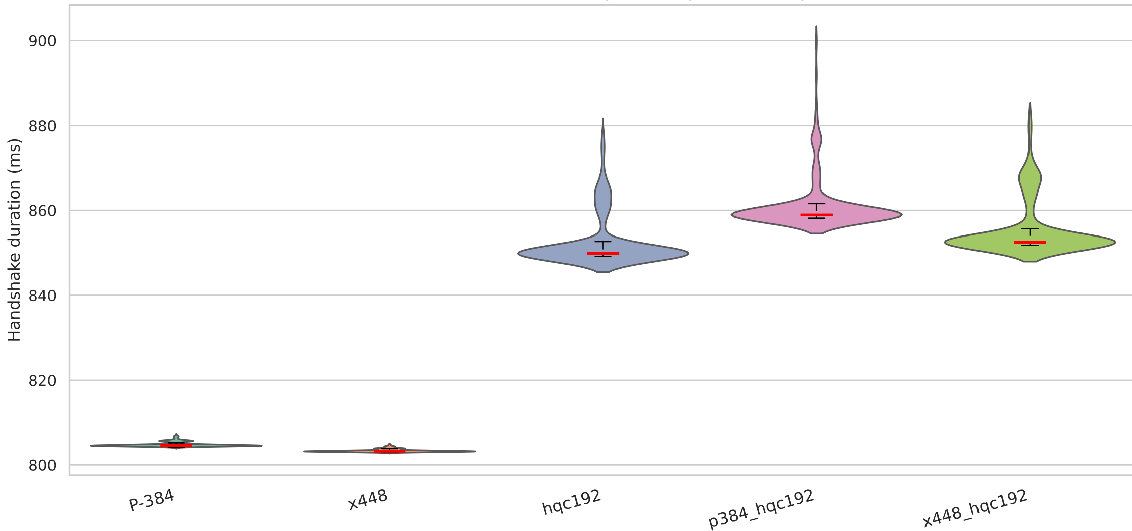
Handshake duration on QUIC with mldsa65 signature algorithm — Degraded (200ms/10%)
