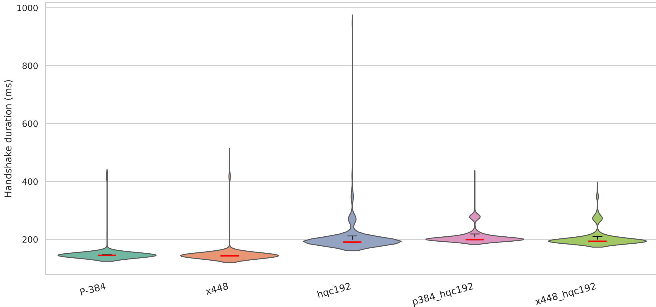
Handshake duration on QUIC with mlds65 signature algorithm — Local YDE (35ms/2%)
