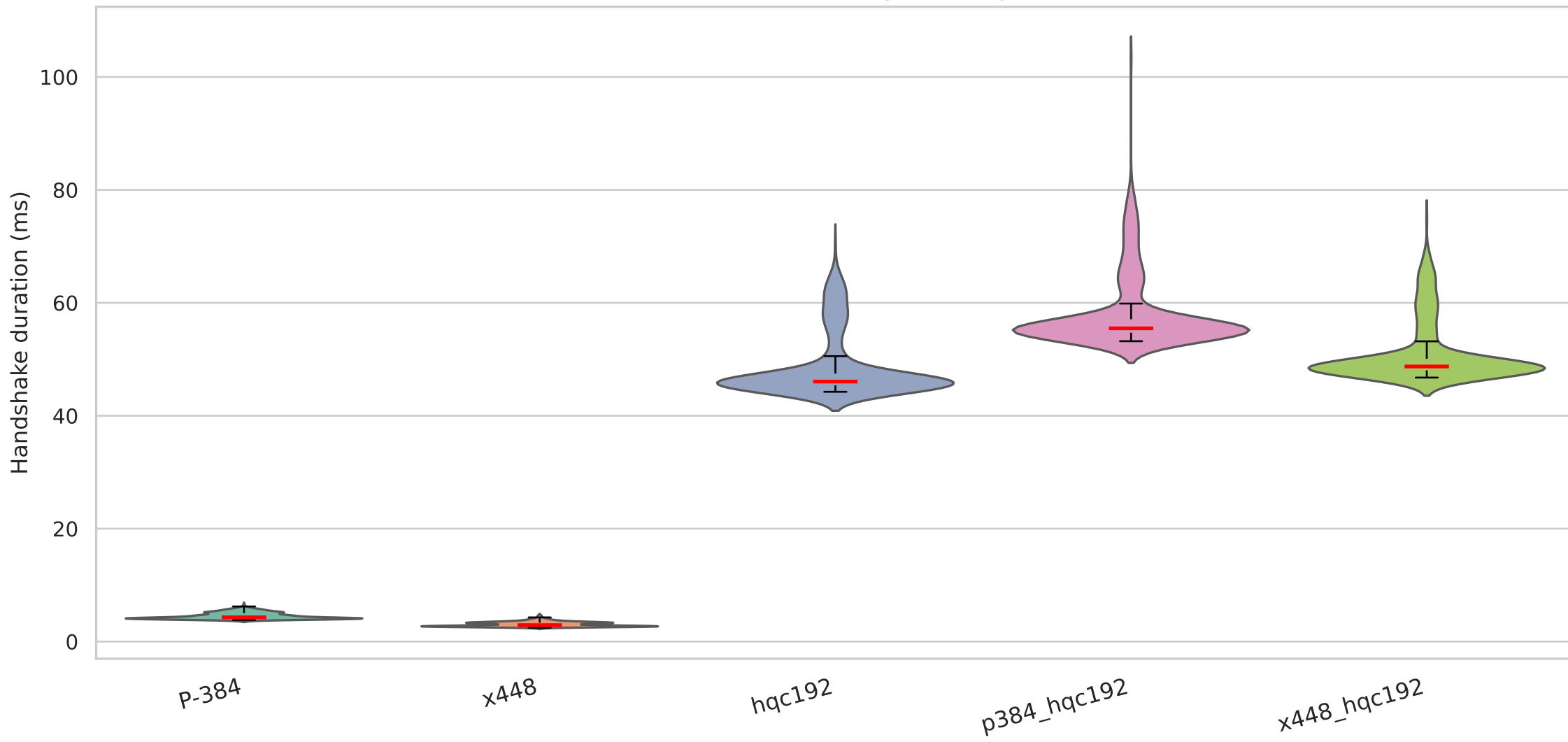
Handshake duration on QUIC with mldsa65 signature algorithm — ideal conditions
