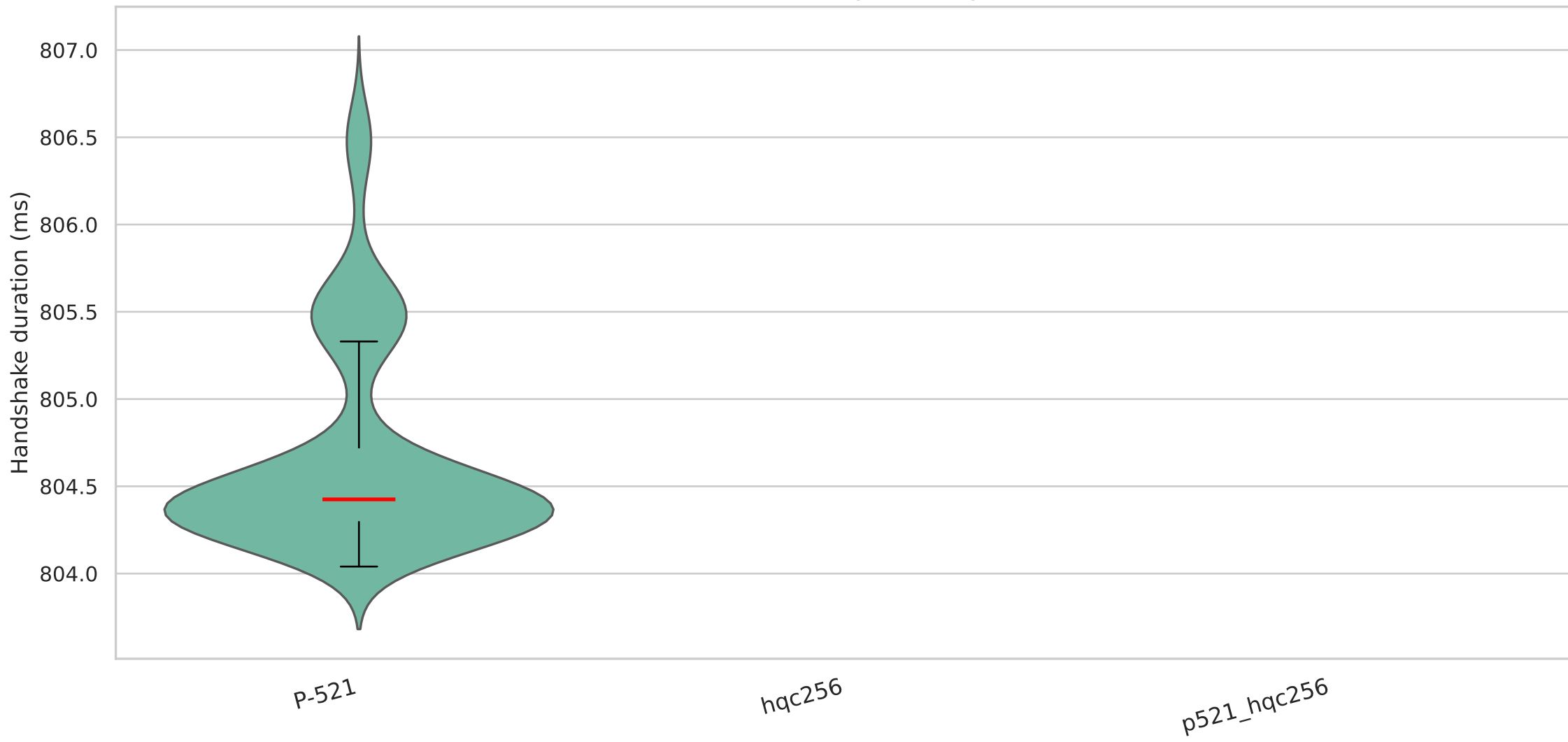
Handshake duration on QUIC with mldsa87 signature algorithm — Backbone (200ms/4%)
