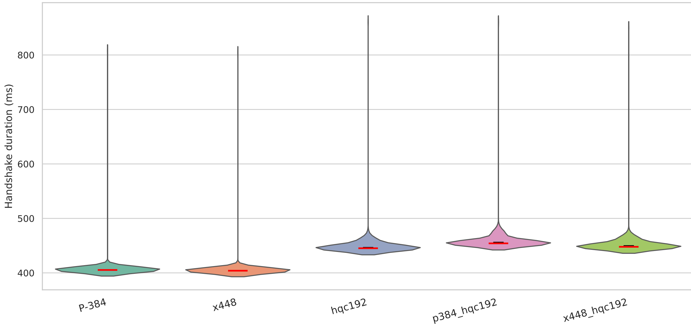
Handshake duration on QUIC with secp384r1 signature algorithm — Backbone (200ms/4%)
