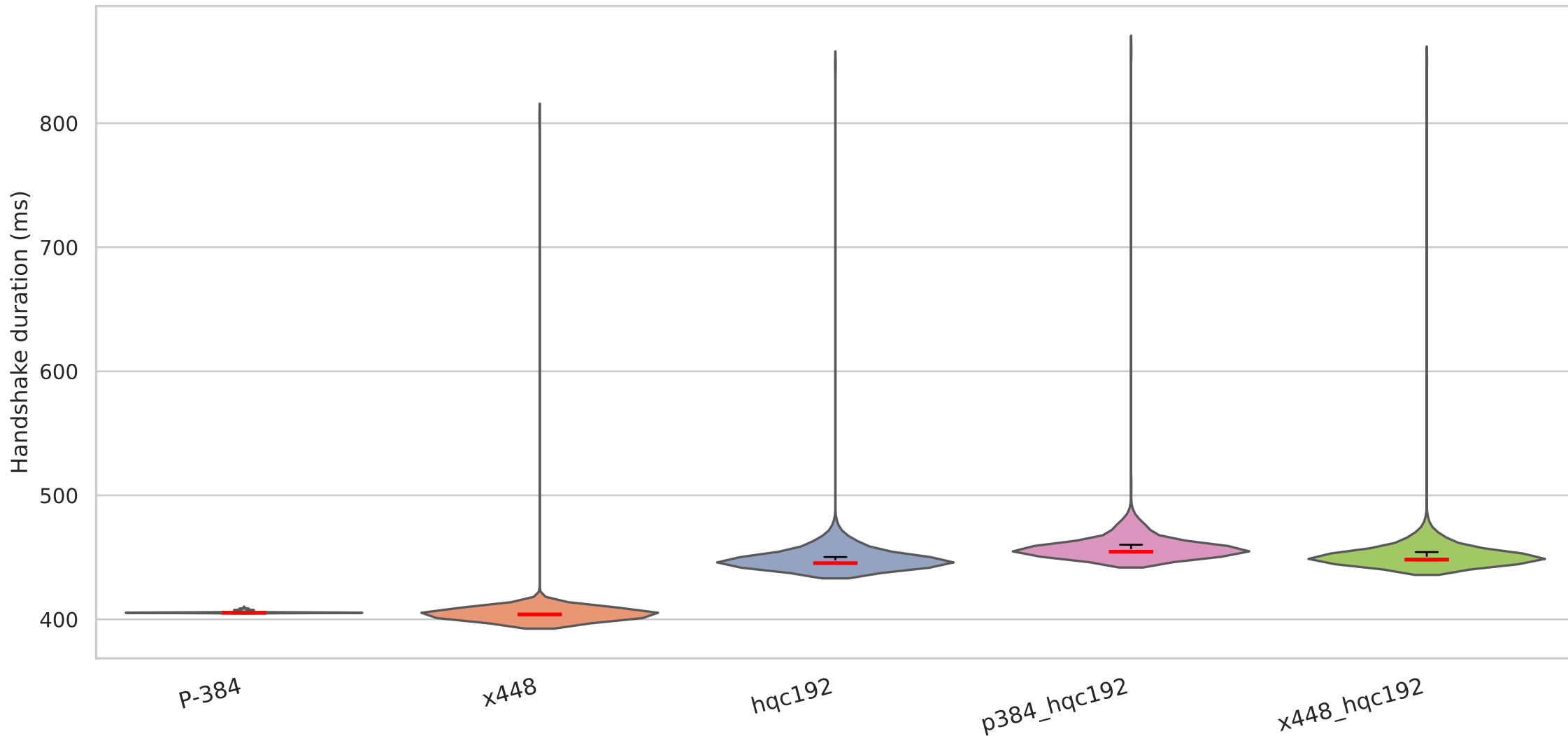
Handshake duration on QUIC with secp384r1 signature algorithm — Degraded (200ms/10%)
