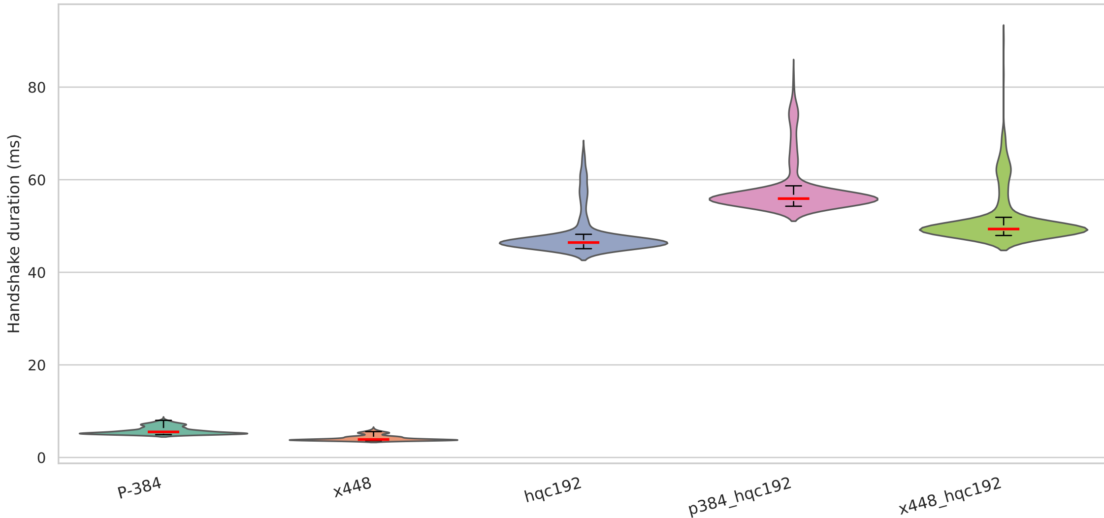
Handshake duration on QUIC with secp384r1 signature algorithm — ideal conditions
