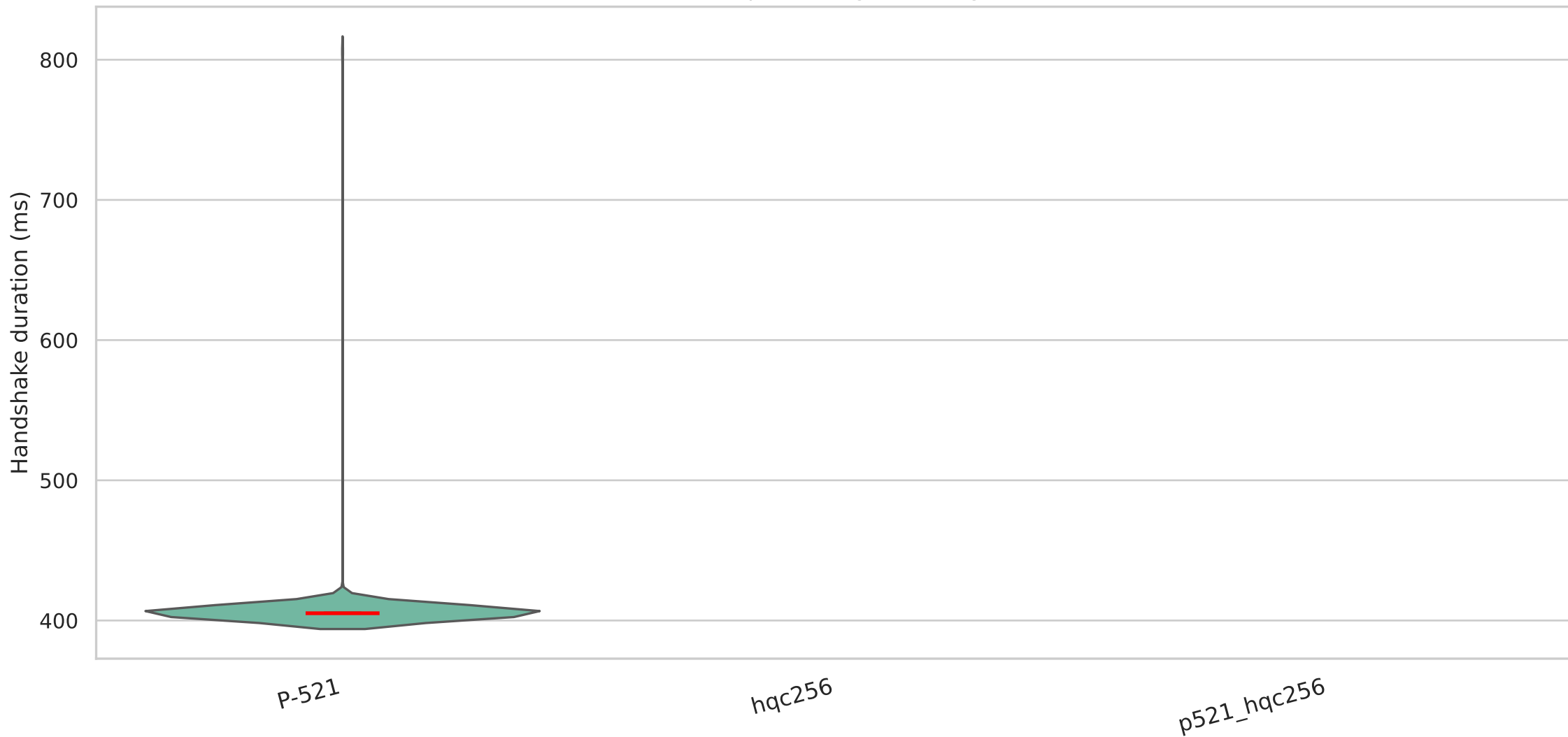
Handshake duration on QUIC with secp521r1 signature algorithm — Backbone (200ms/4%)
