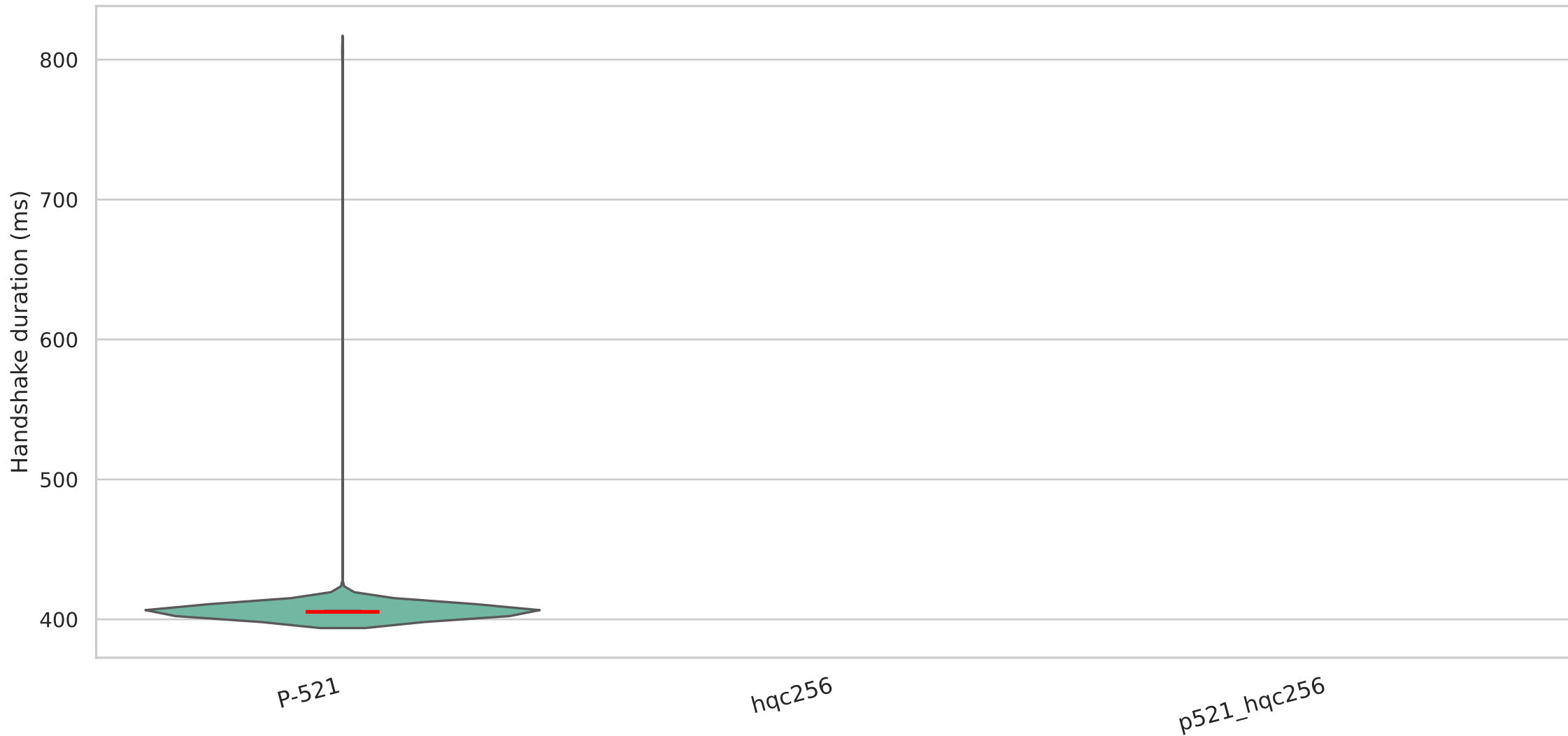
Handshake duration on QUIC with secp521r1 signature algorithm — Degraded (200ms/10%)
