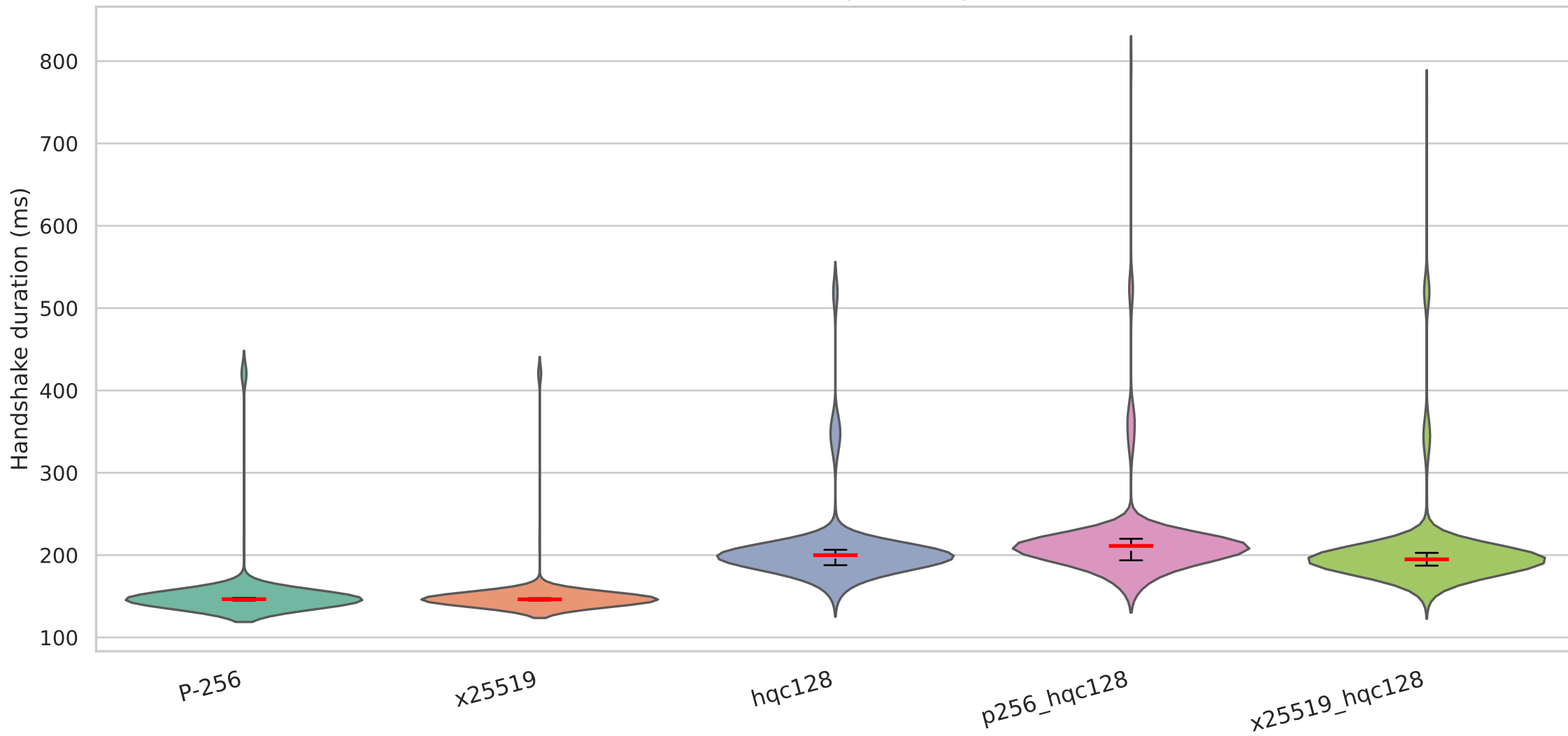
Handshake duration on TLS with ed25519 signature algorithm — Local YDE (35ms/2%)
