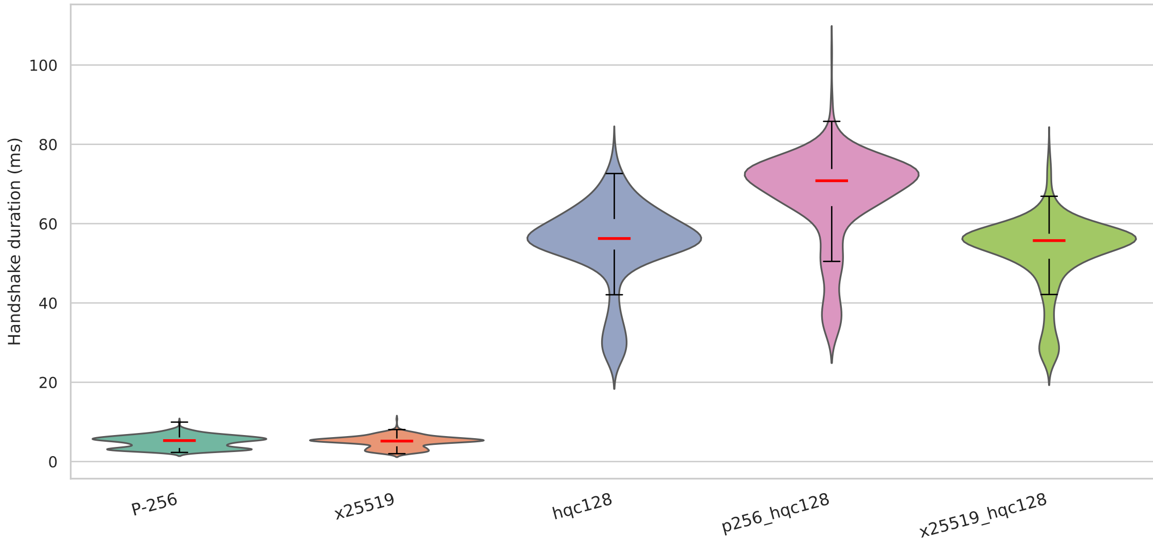
Handshake duration on TLS with ed25519 signature algorithm — ideal conditions
