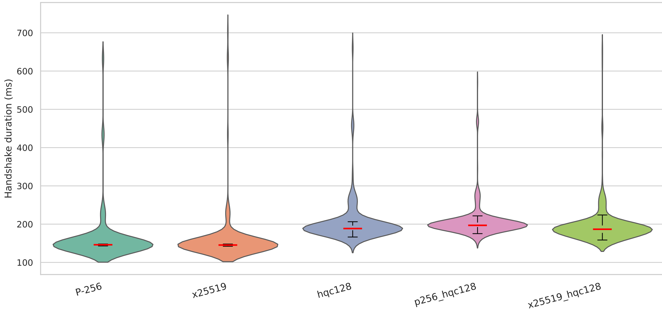
Handshake duration on TLS with mldsa44 signature algorithm — Local YDE (35ms/2%)
