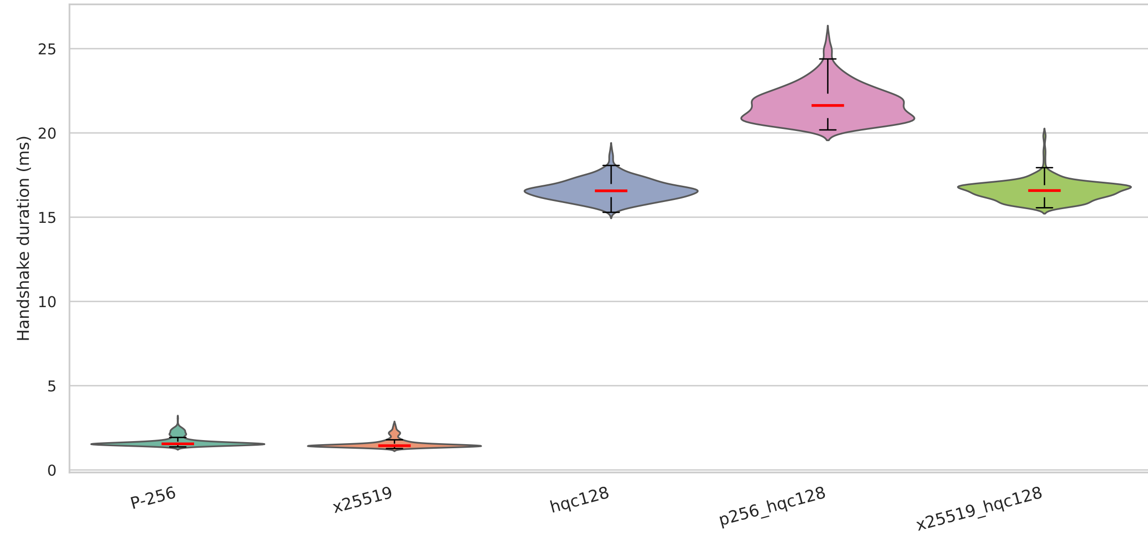
Handshake duration on TLS with mldsa44 signature algorithm — ideal conditions
