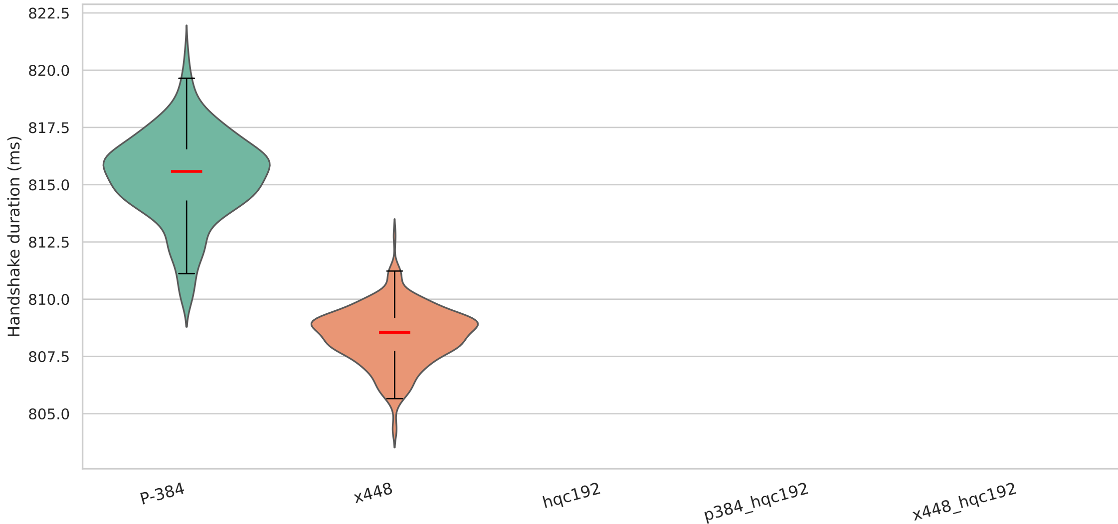
Handshake duration on TLS with mldsa65 signature algorithm — Degraded (200ms/10%)
