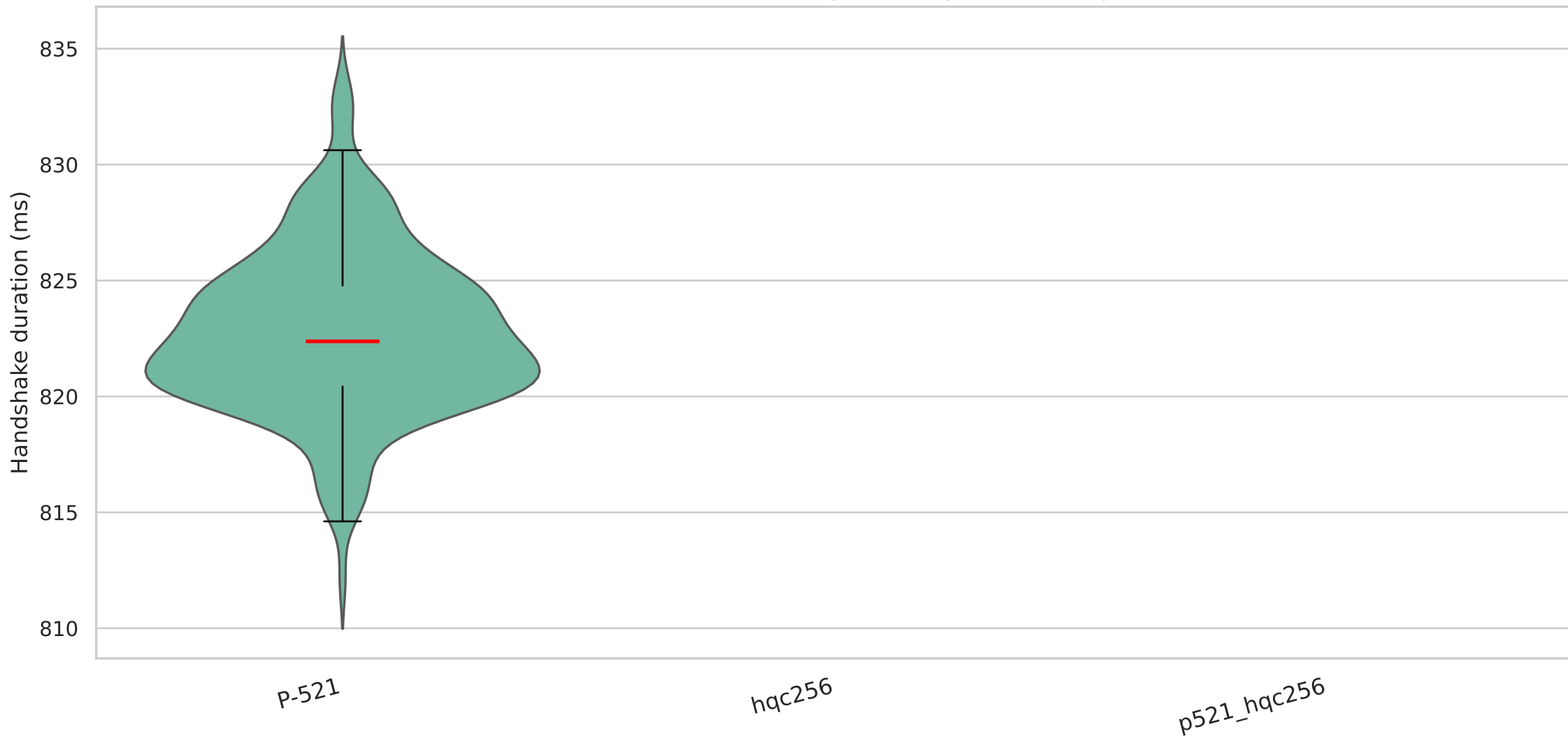
Handshake duration on TLS with mldsa87 signature algorithm — Degraded (200ms/10%)
