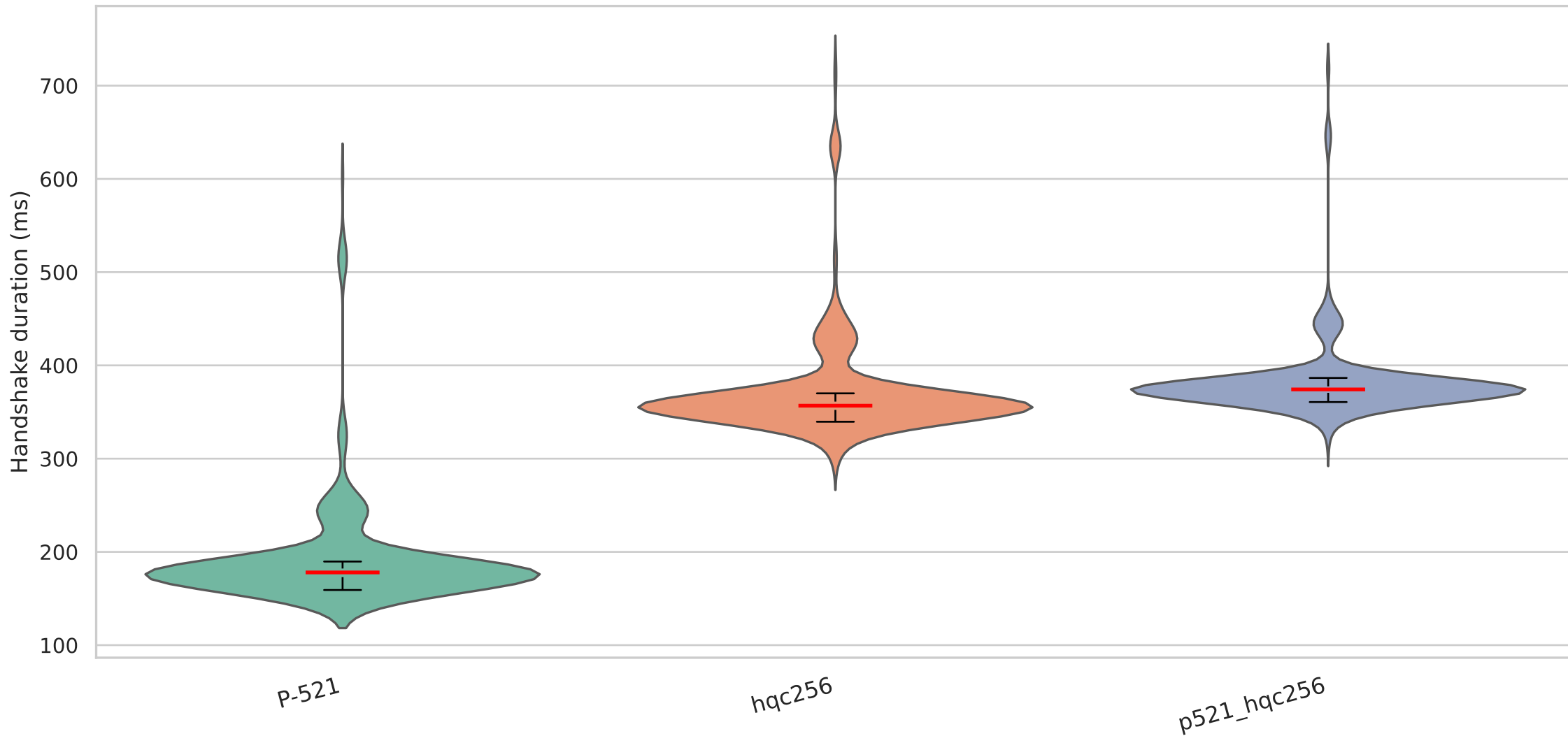
Handshake duration on TLS with mldsa87 signature algorithm — Local YDE (35ms/2%)
