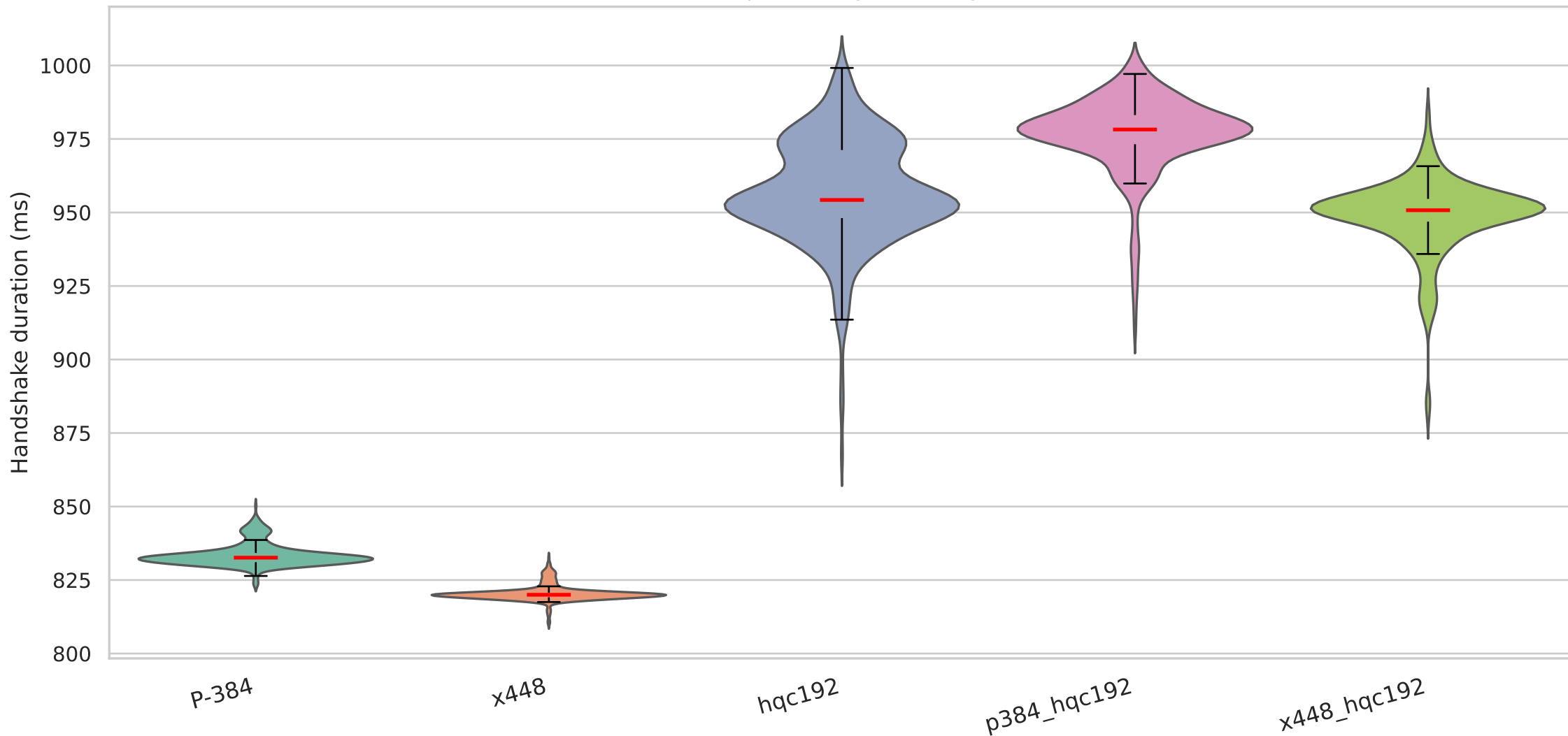
Handshake duration on TLS with secp384r1 signature algorithm — Backbone (200ms/4%)
