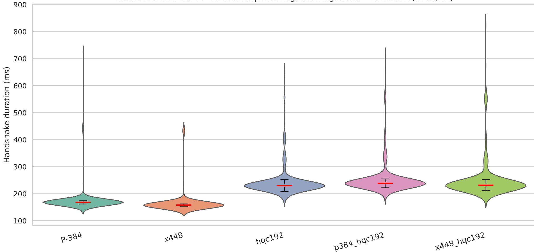
Handshake duration on TLS with secp384r1 signature algorithm — Local YDE (35ms/2%)
