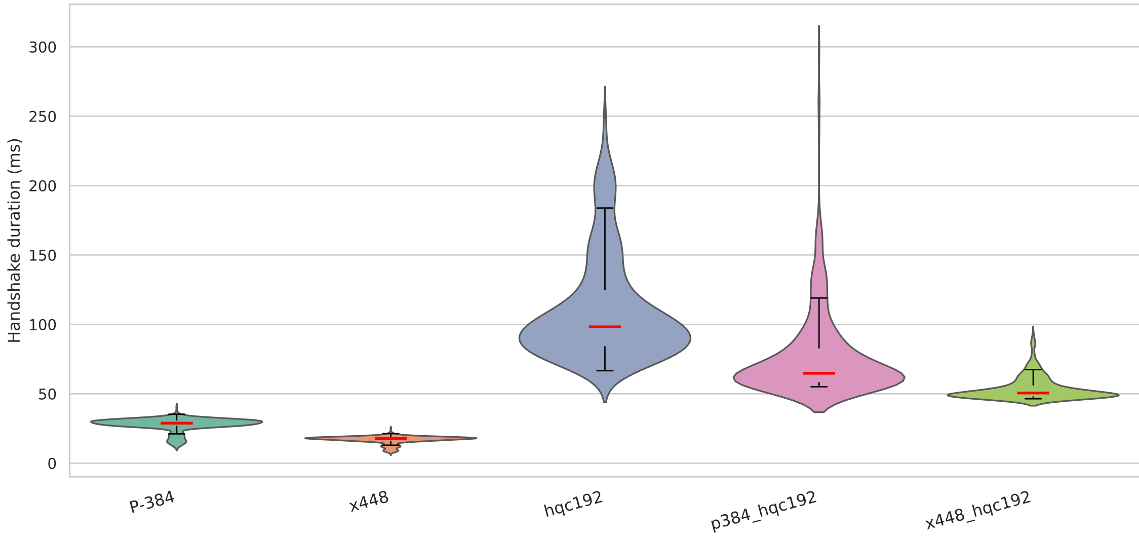
Handshake duration on TLS with secp384r1 signature algorithm — ideal conditions
