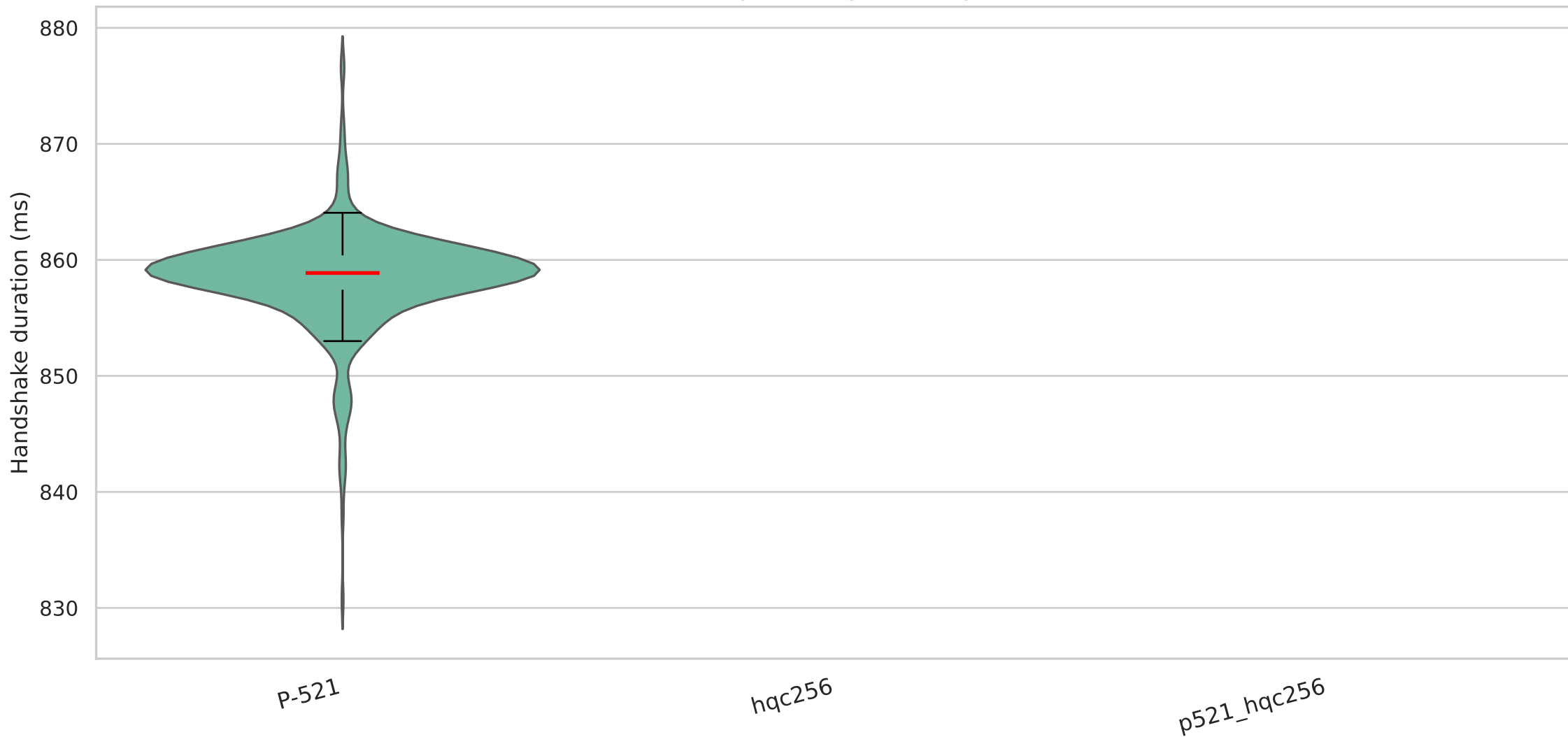
Handshake duration on TLS with secp521r1 signature algorithm — Backbone (200ms/4%)
