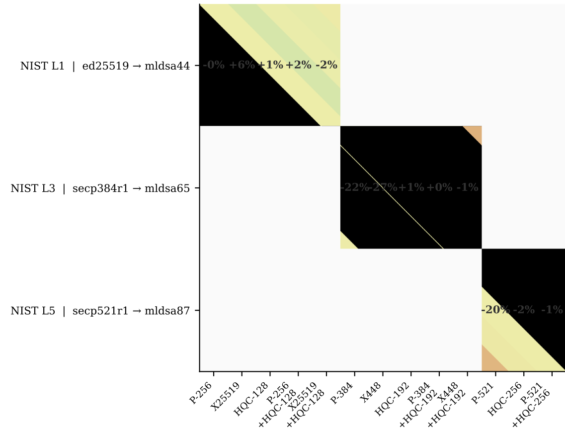
QUIC
