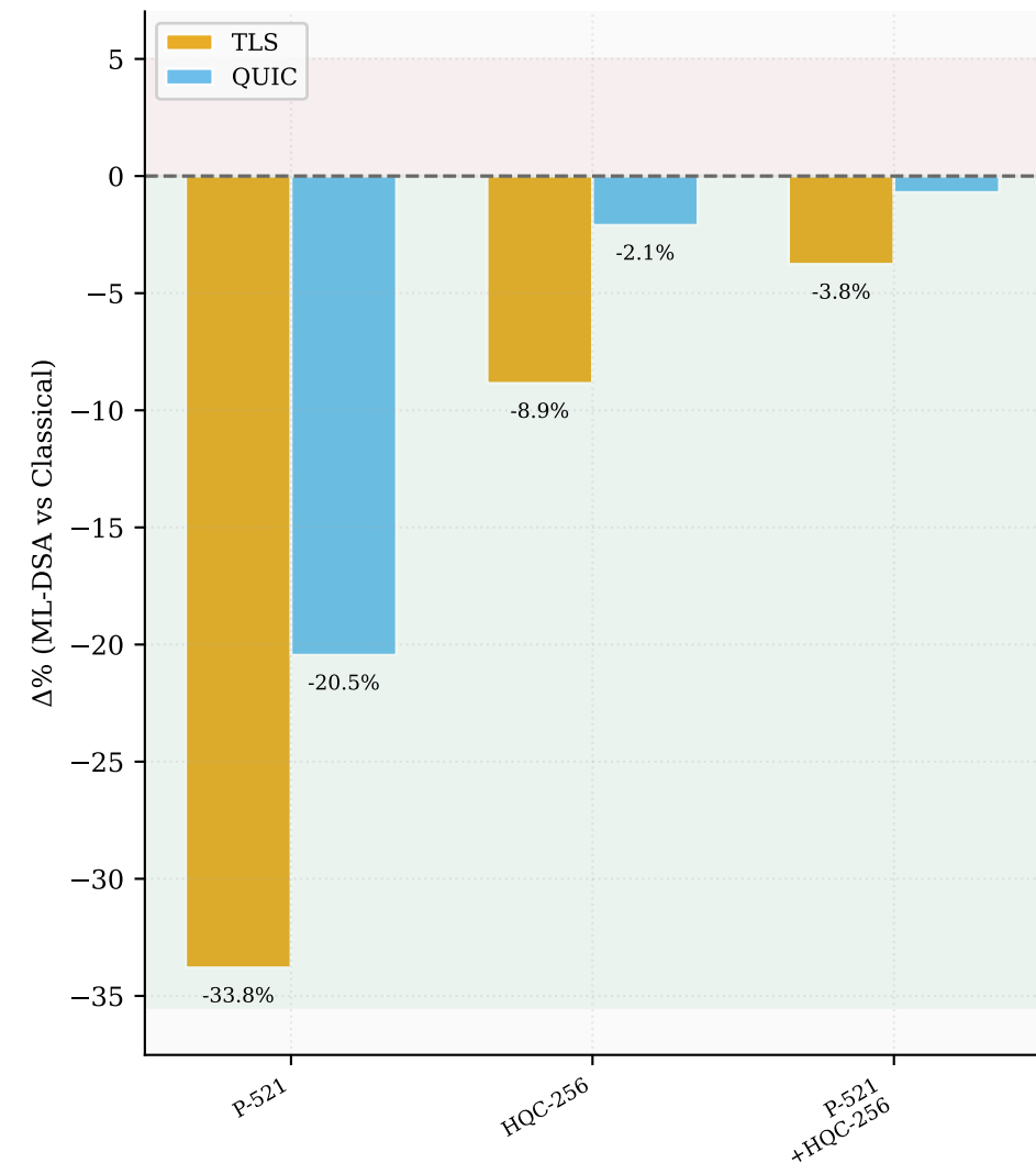
L5 — secp521r1 → mldsa87
