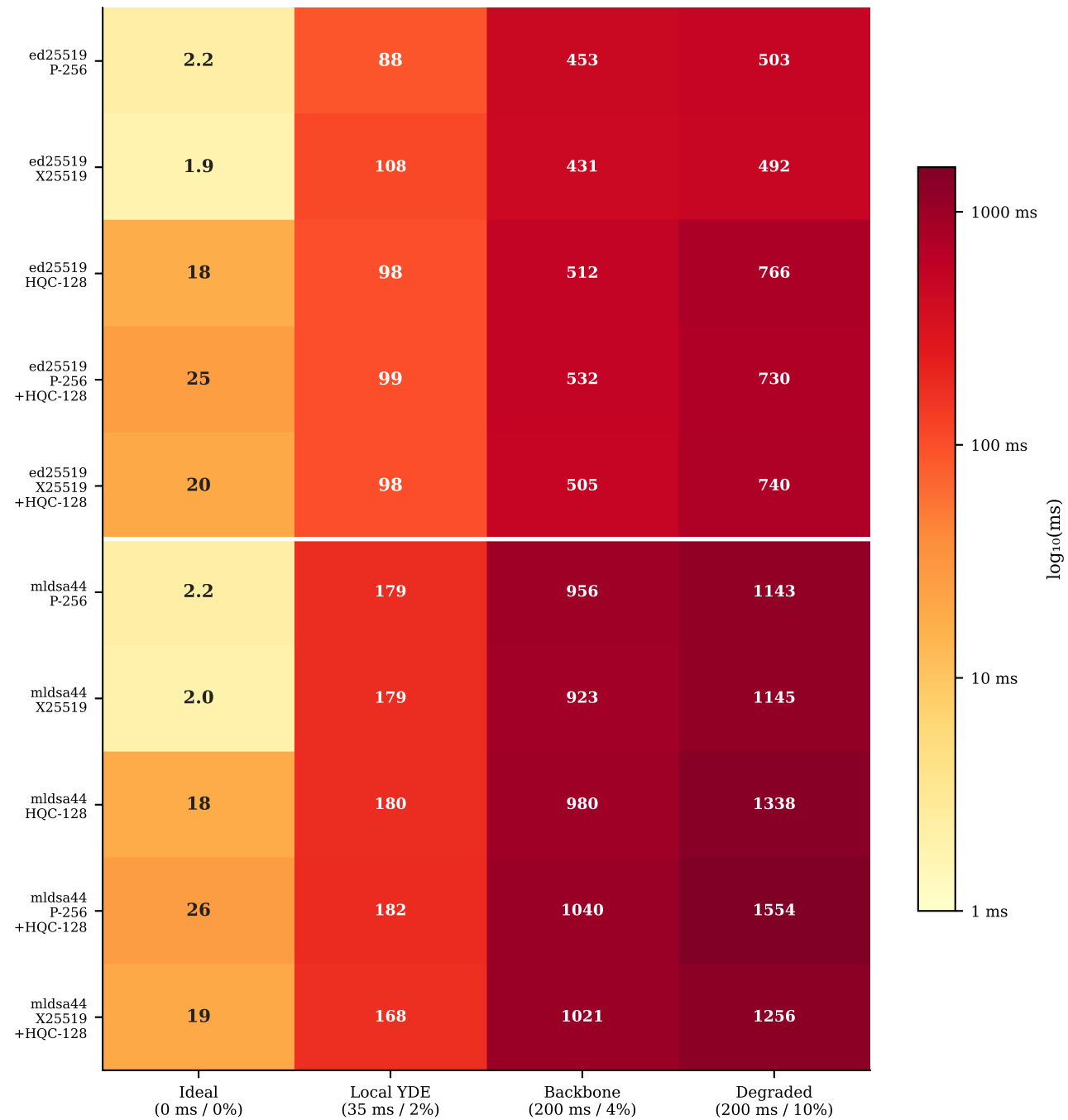
QUIC
