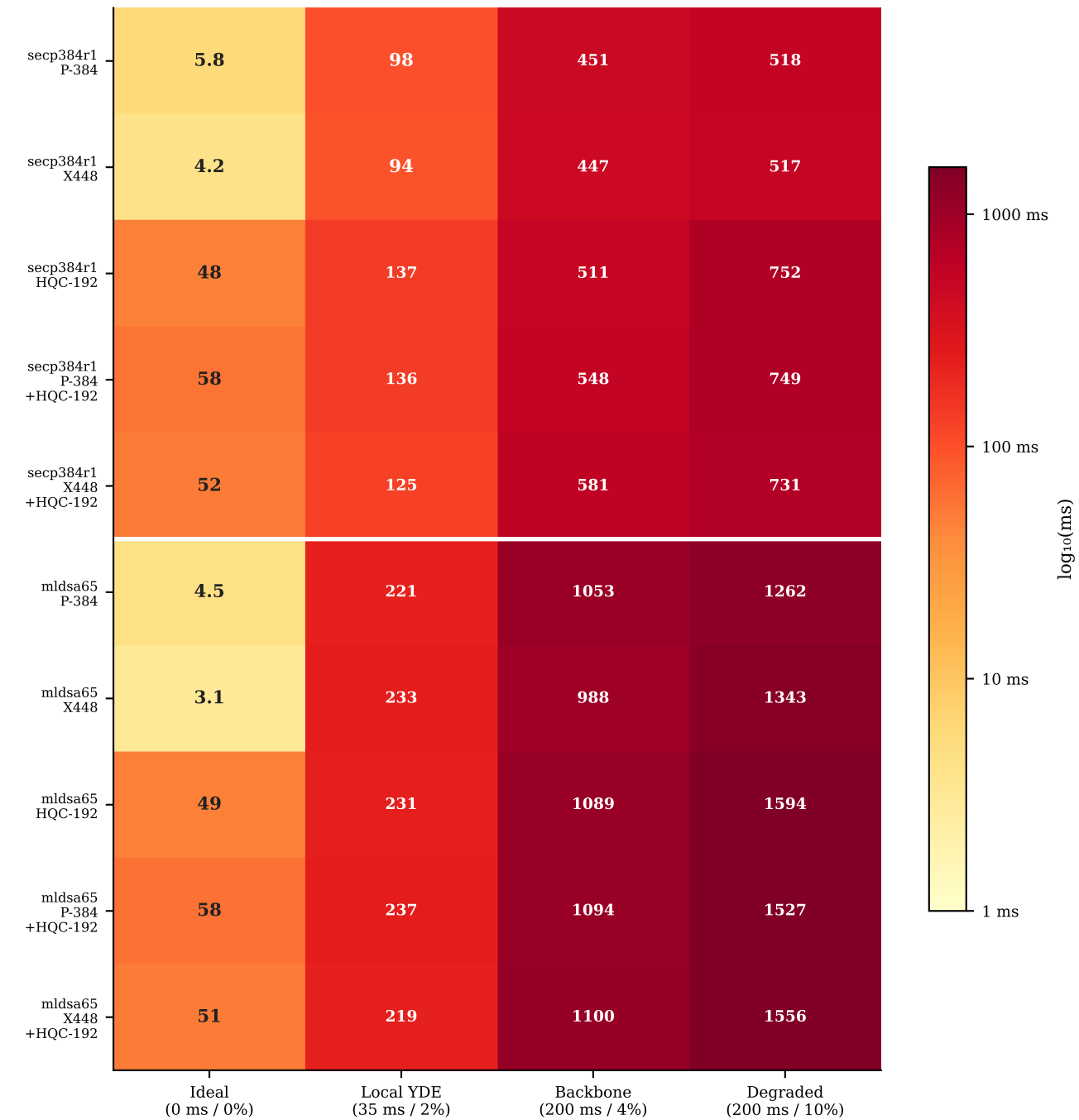
QUIC
