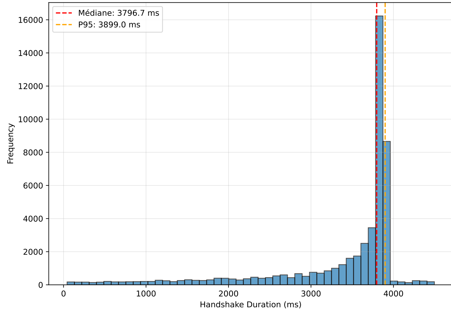
Distribution globale — mldsa65 × hqc192
