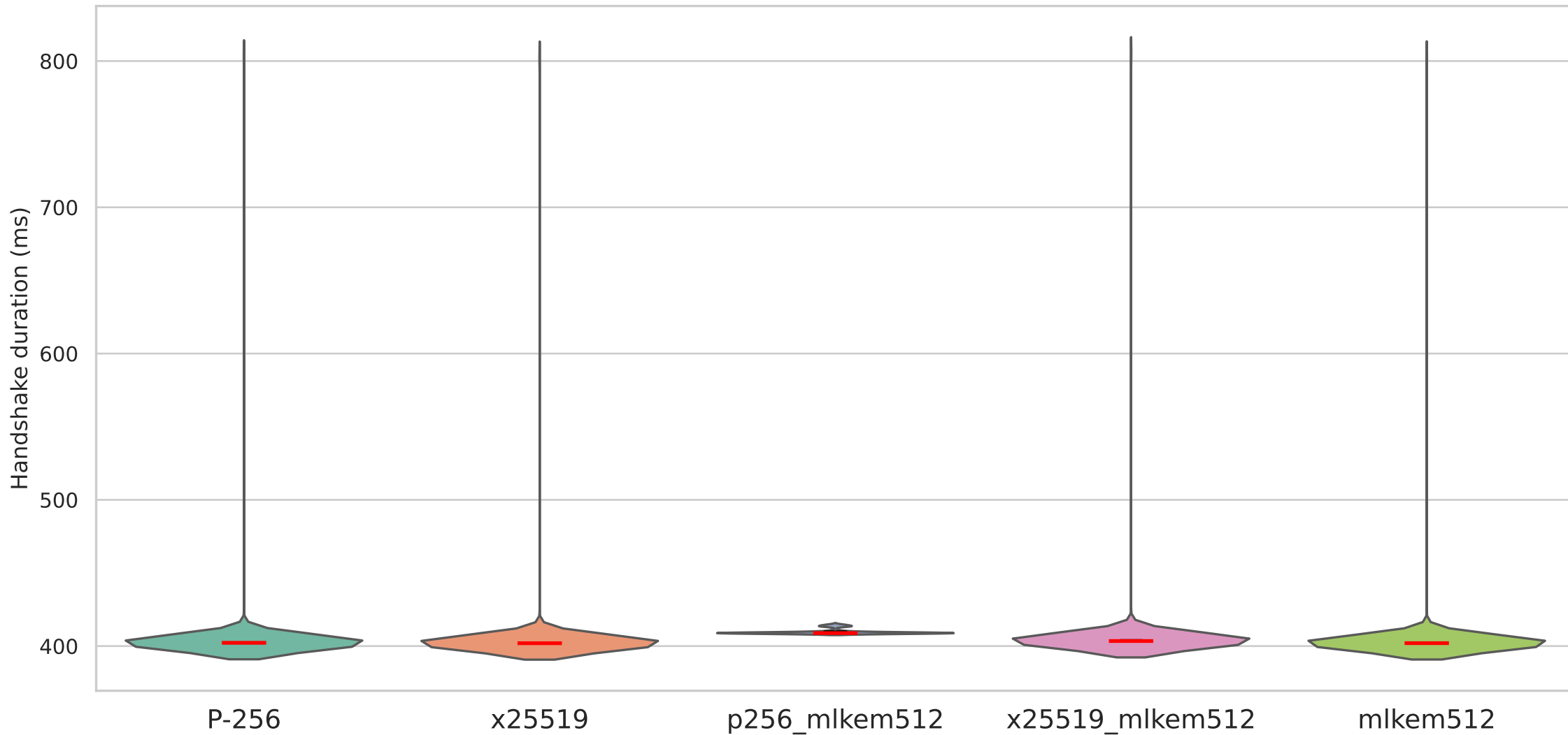
Handshake duration on QUIC with ed25519 signature algorithm — Backbone (200ms/4%)
