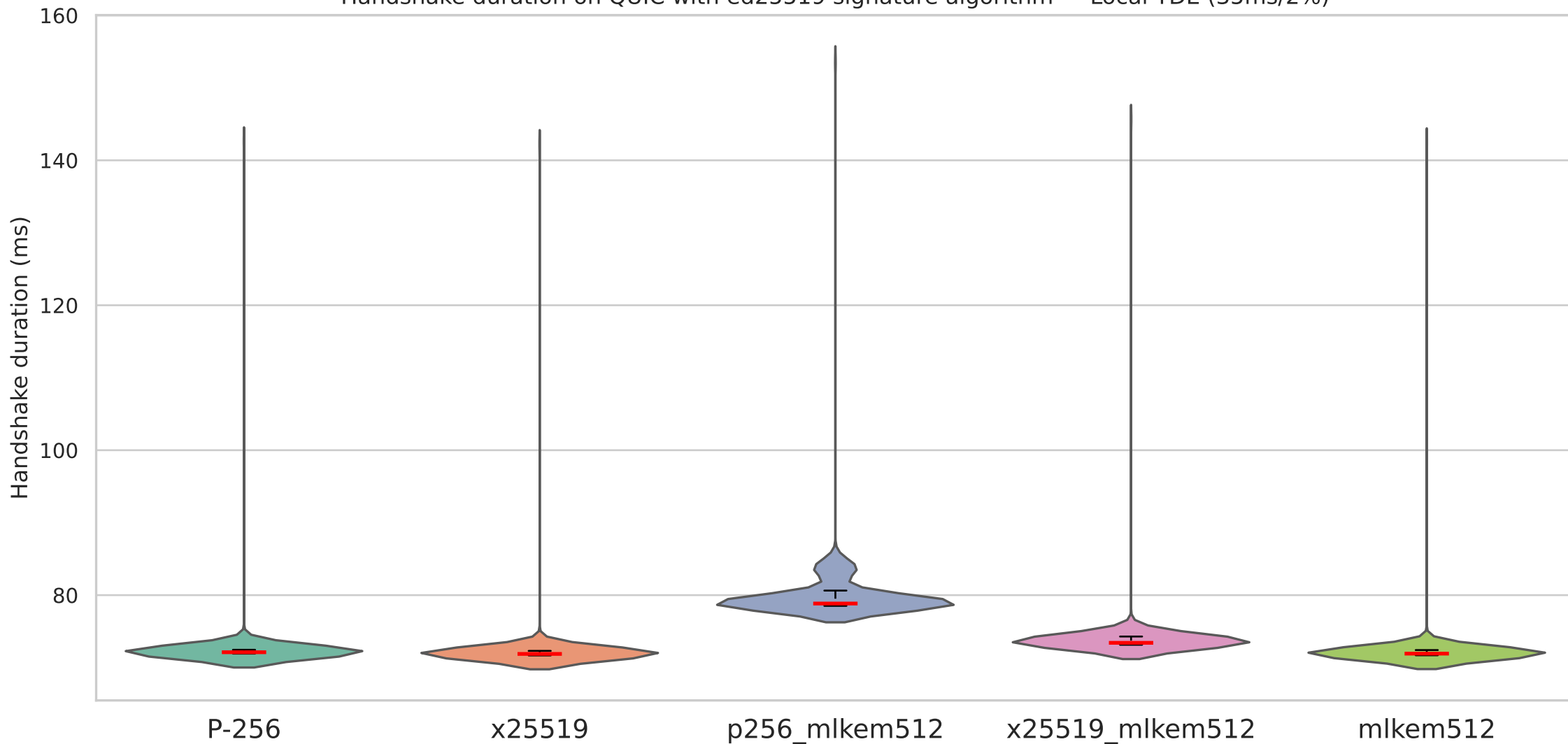
Handshake duration on QUIC with ed25519 signature algorithm — Local YDE (35ms/2%)
