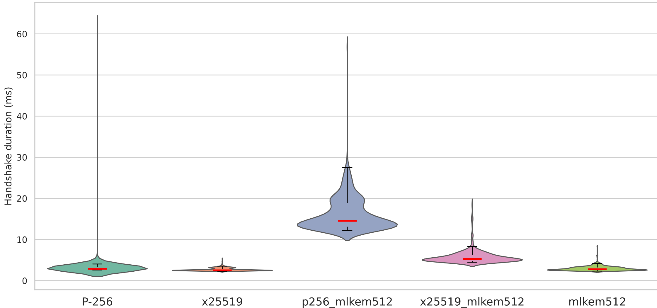
Handshake duration on QUIC with ed25519 signature algorithm — ideal conditions
