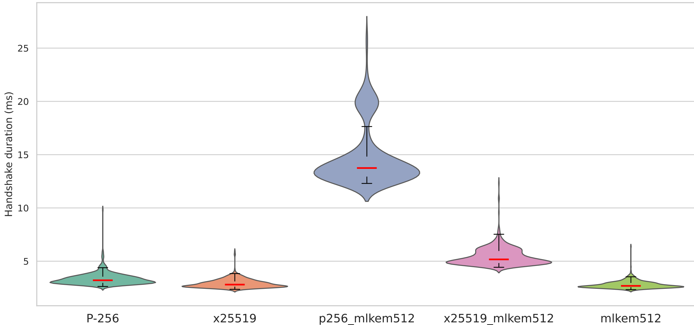
Handshake duration on QUIC with mldsa44 signature algorithm — ideal conditions
