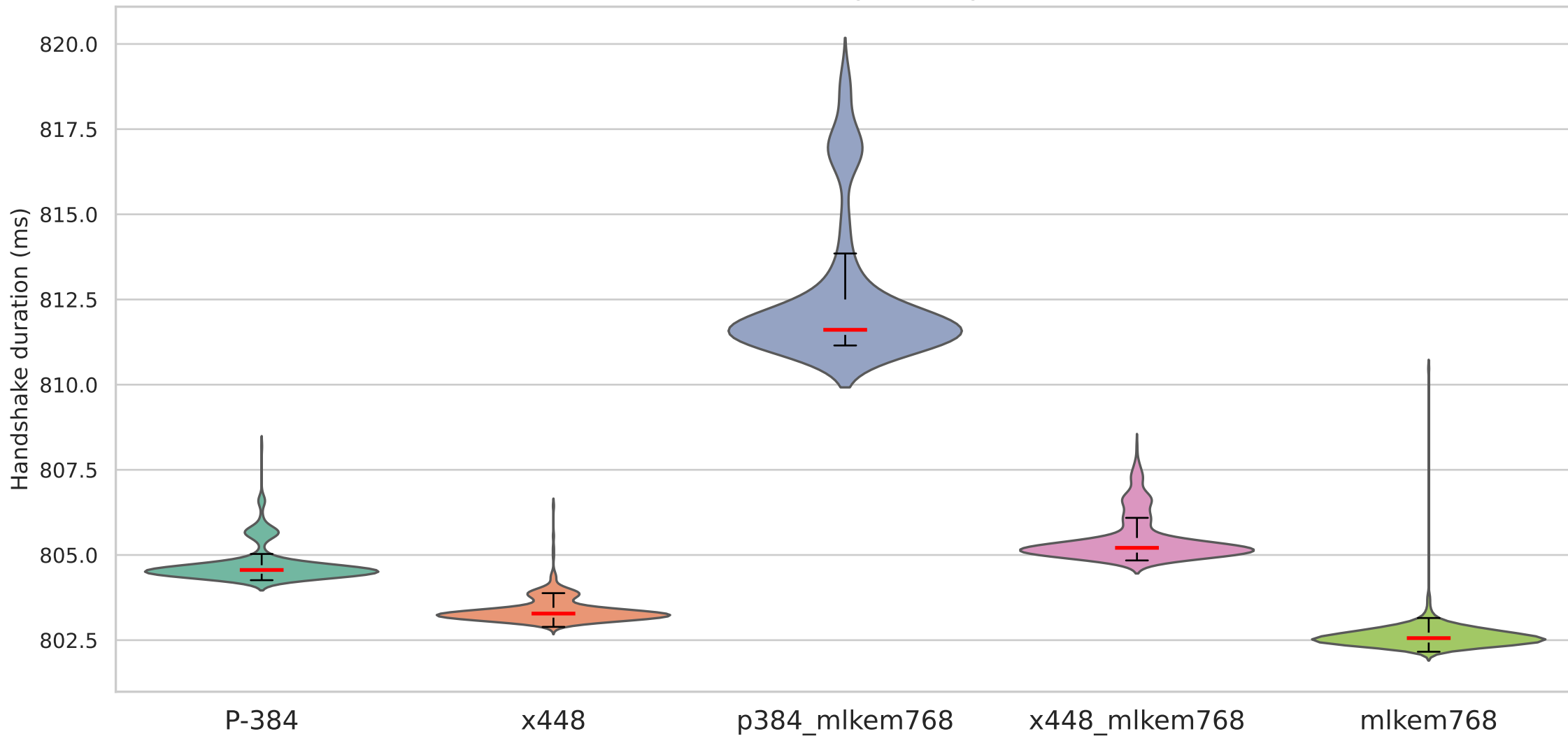
Handshake duration on QUIC with mlrsa65 signature algorithm — Backbone (200ms/4%)
