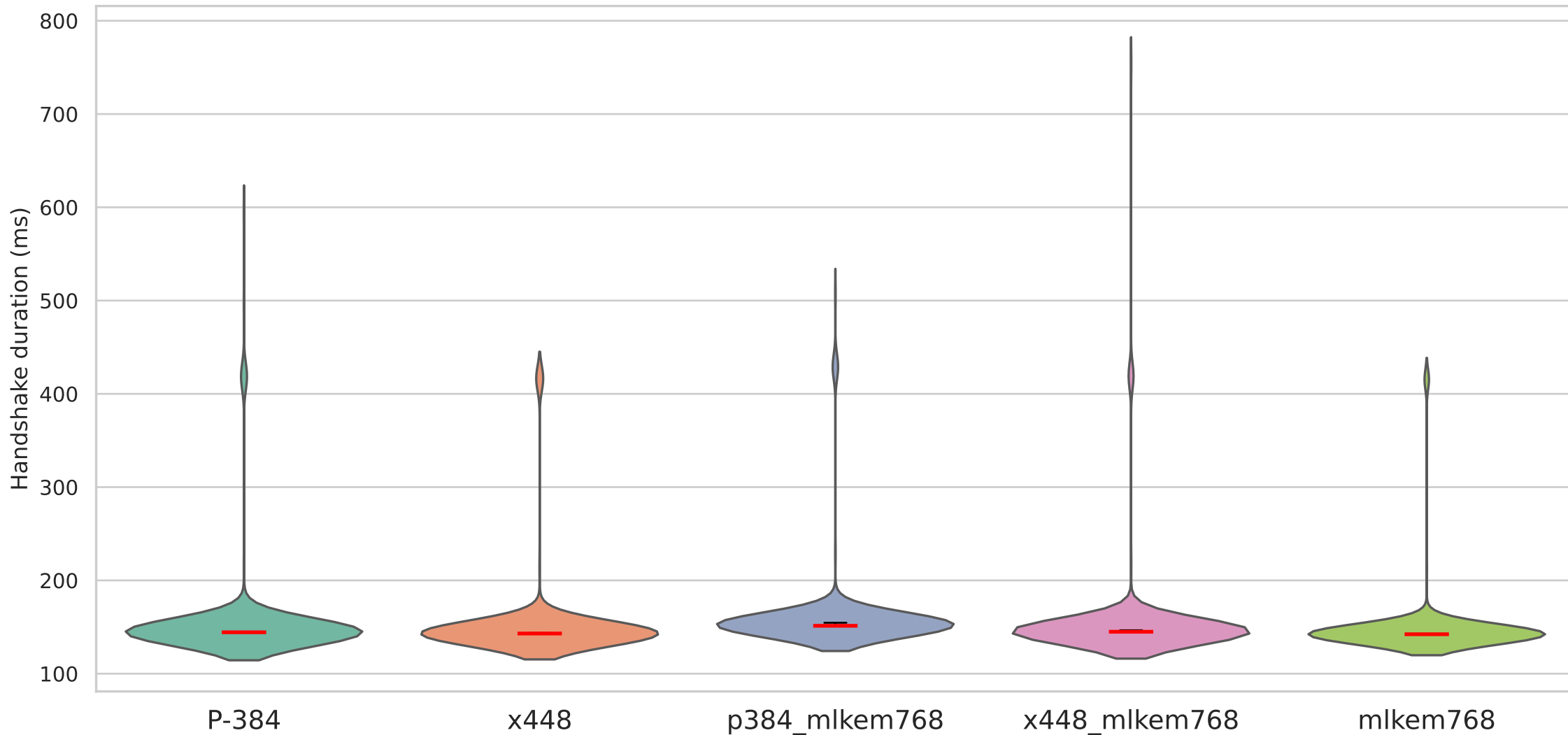
Handshake duration on QUIC with mldsa65 signature algorithm — Local YDE (35ms/2%)
