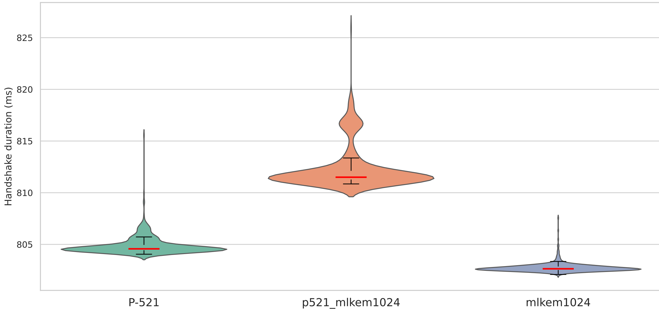
Handshake duration on QUIC with mlds87 signature algorithm — Backbone (200ms/4%)
