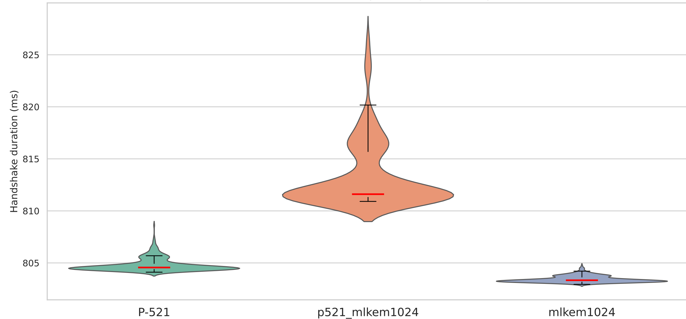
Handshake duration on QUIC with mlds87 signature algorithm — Degraded (200ms/10%)
