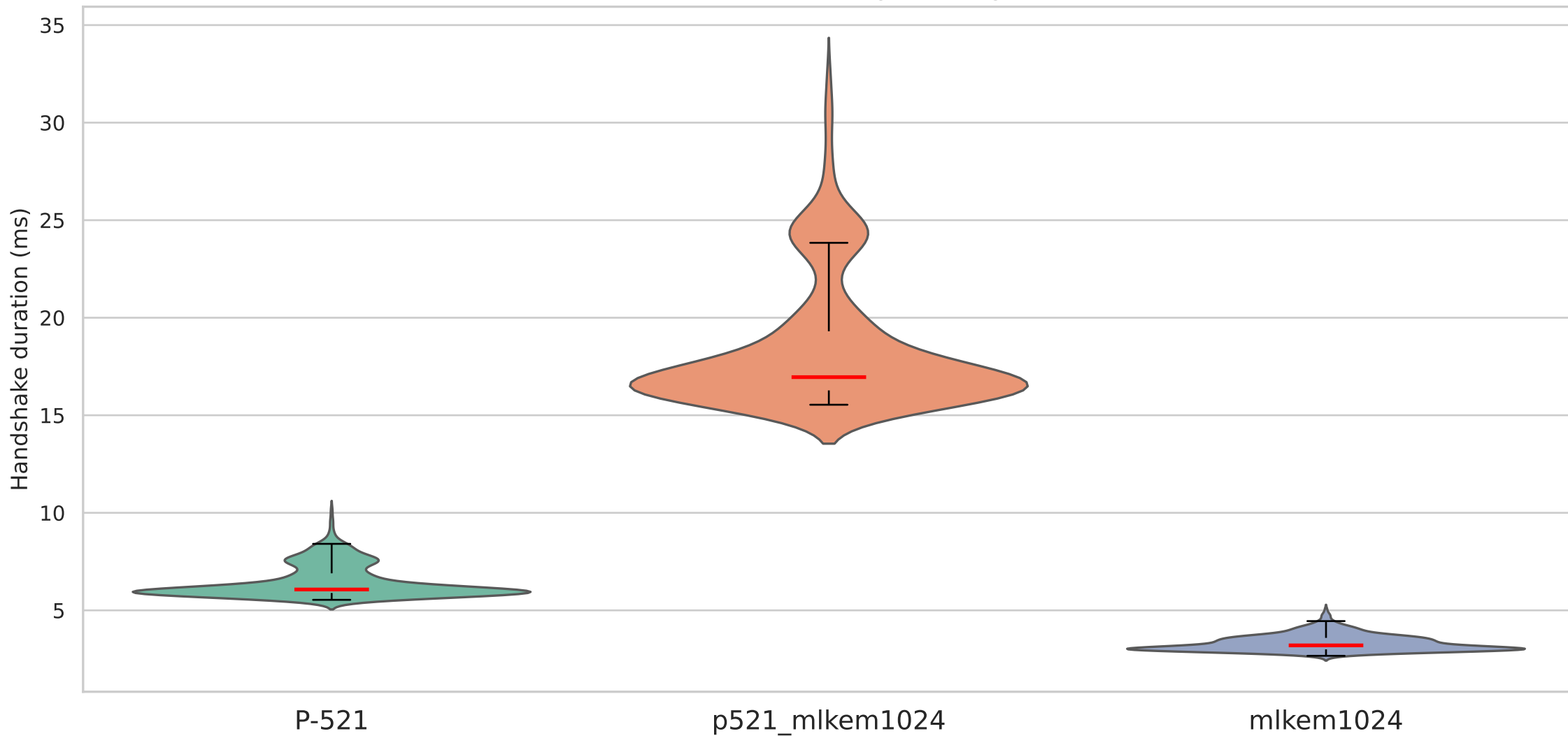
Handshake duration on QUIC with mldsa87 signature algorithm — ideal conditions
