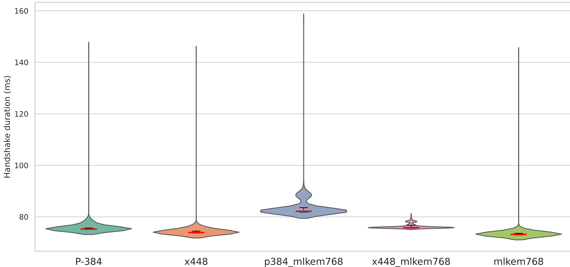
Handshake duration on QUIC with secp384r1 signature algorithm — Local YDE (35ms/2%)
