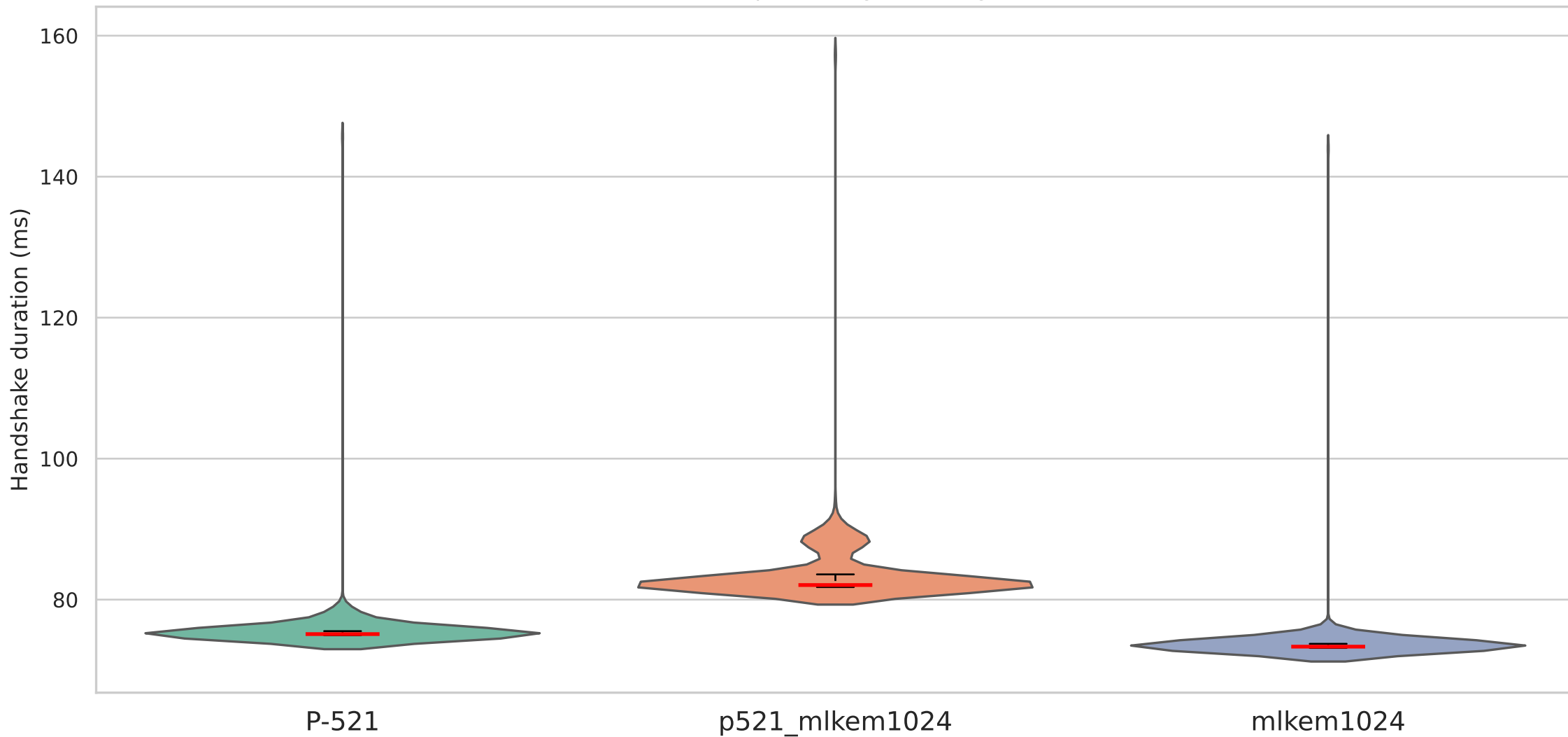
Handshake duration on QUIC with secp521r1 signature algorithm — Local YDE (35ms/2%)
