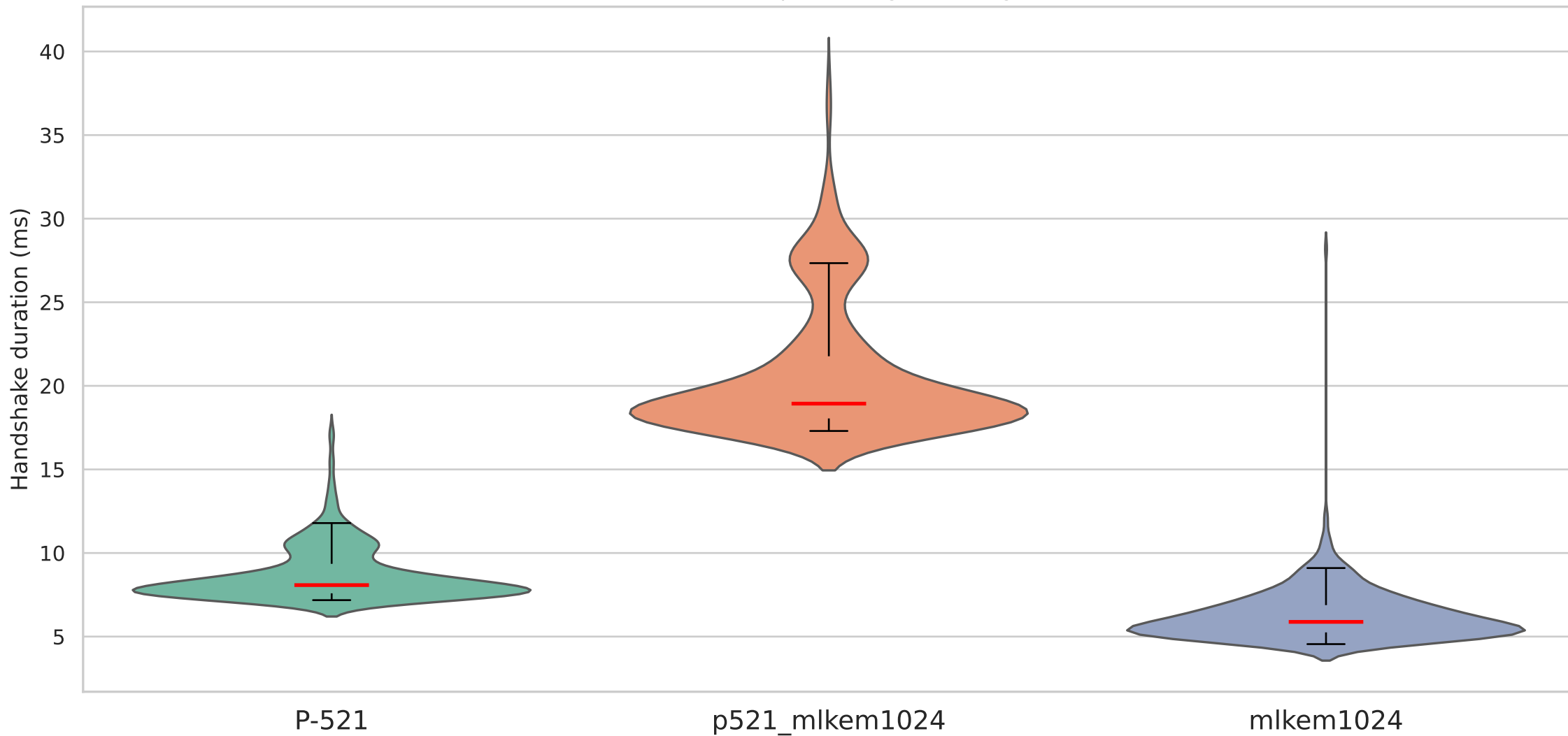
Handshake duration on QUIC with secp521r1 signature algorithm — ideal conditions
