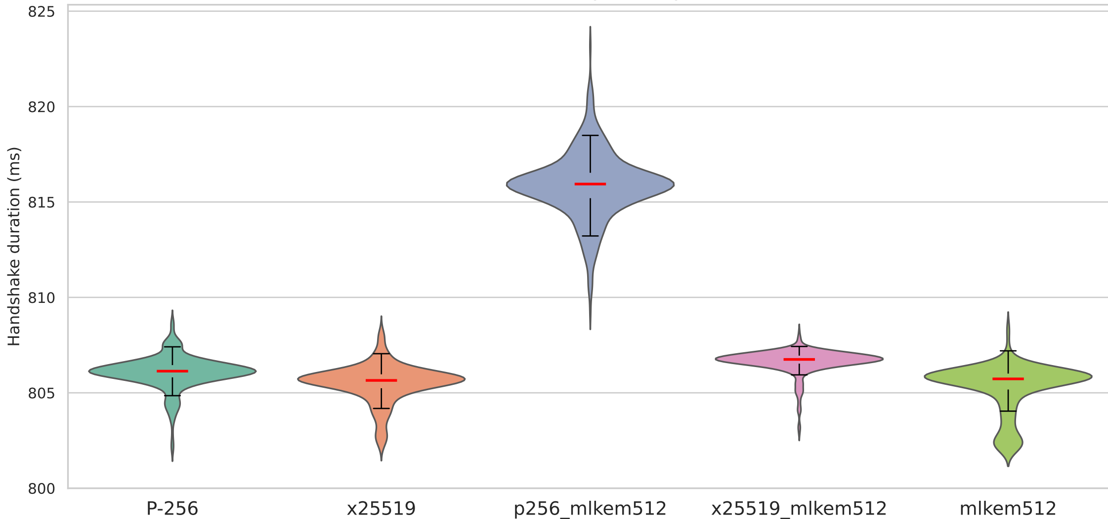
Handshake duration on TLS with ed25519 signature algorithm — Backbone (200ms/4%)
