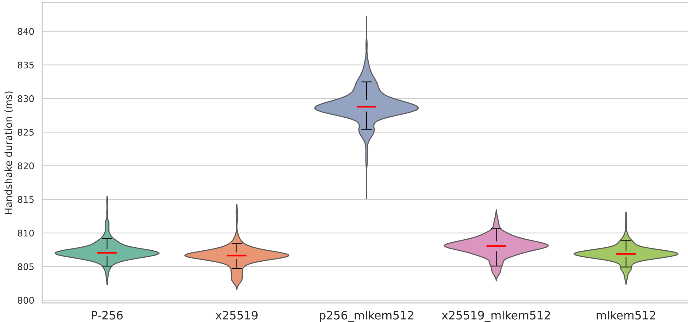
Handshake duration on TLS with ed25519 signature algorithm — Degraded (200ms/10%)
