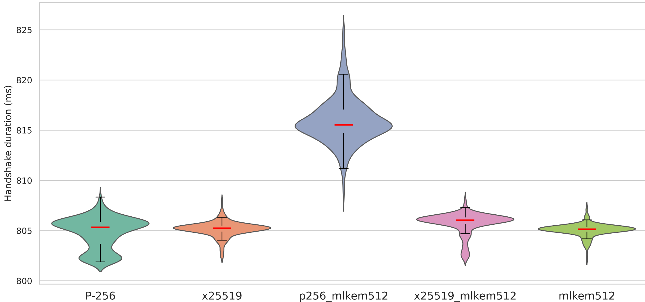
Handshake duration on TLS with mldsa44 signature algorithm — Backbone (200ms/4%)
