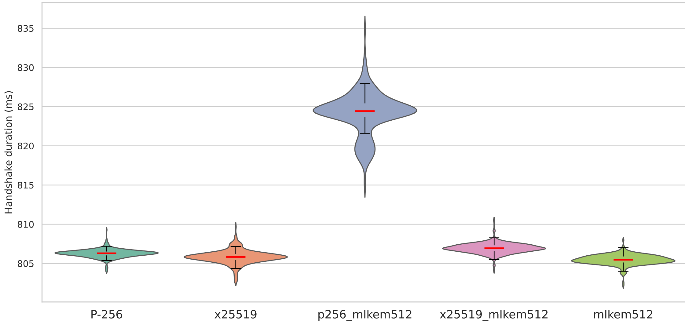
Handshake duration on TLS with mldsa44 signature algorithm — Degraded (200ms/10%)
