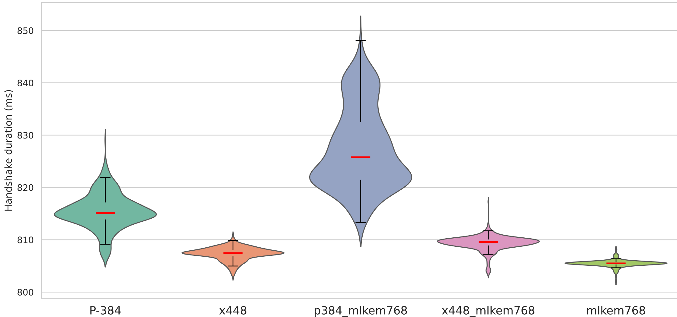
Handshake duration on TLS with mldsa65 signature algorithm — Backbone (200ms/4%)
