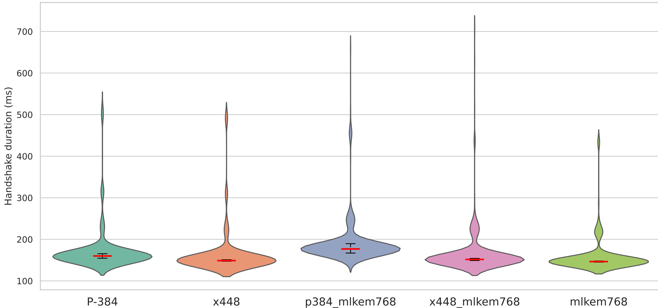
Handshake duration on TLS with mldsa65 signature algorithm — Local YDE (35ms/2%)
