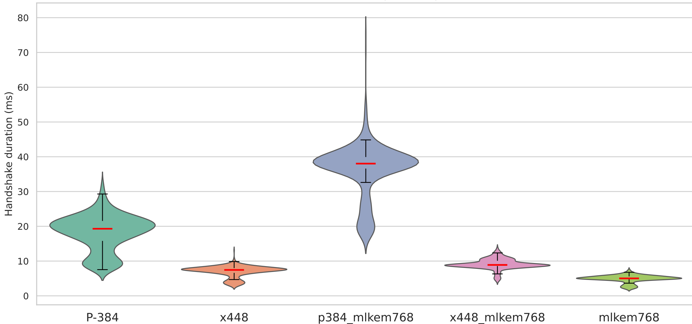
Handshake duration on TLS with mldsa65 signature algorithm — ideal conditions
