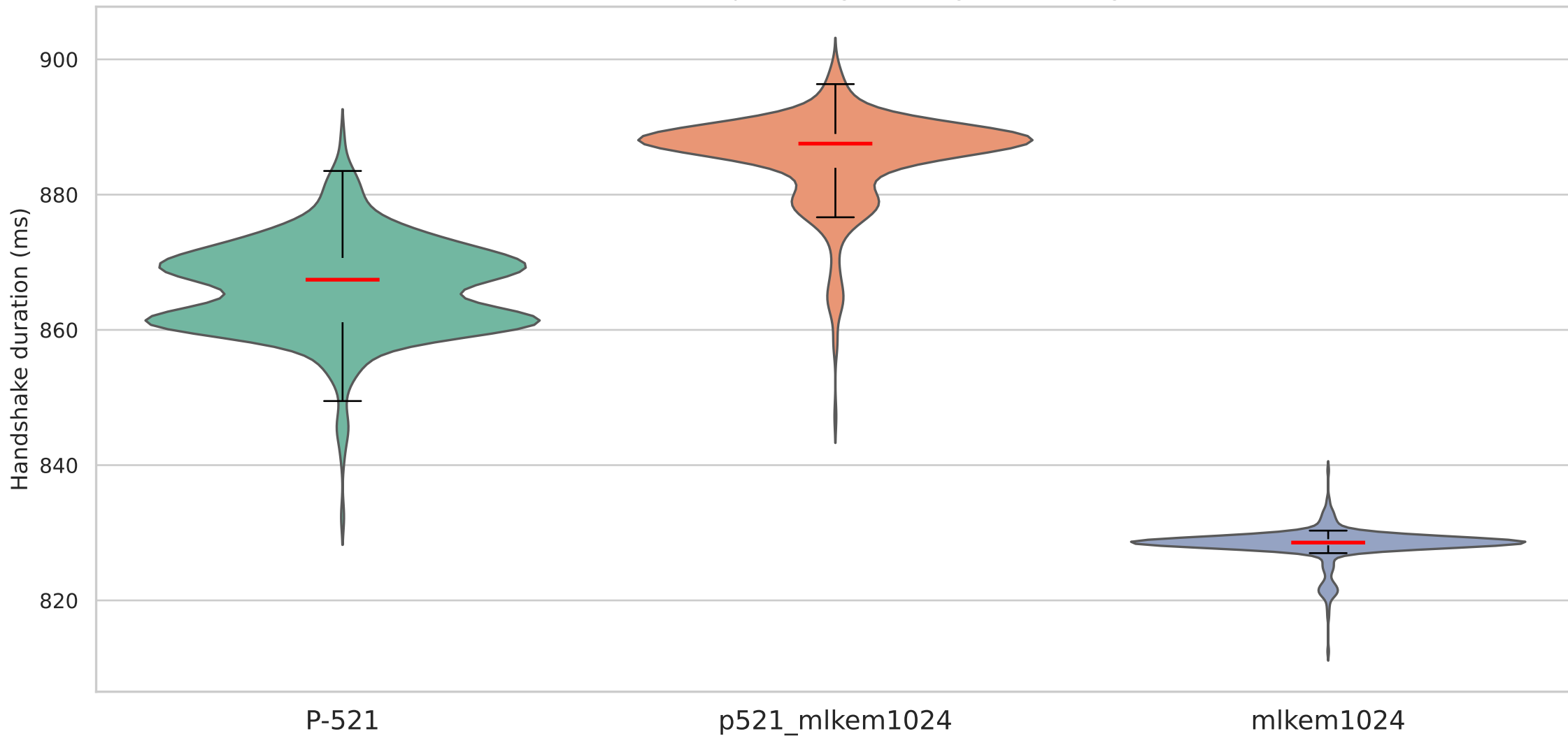
Handshake duration on TLS with secp521r1 signature algorithm — Degraded (200ms/10%)
