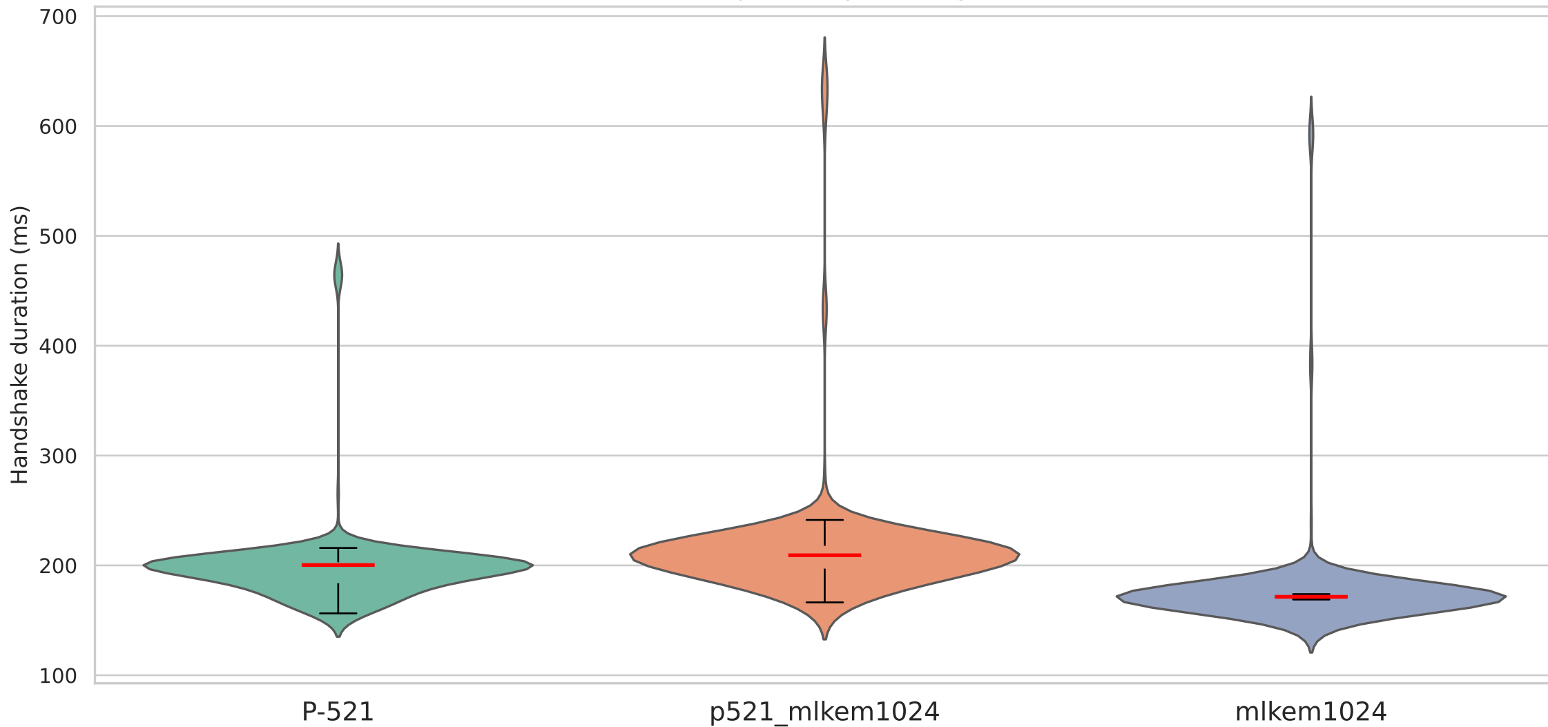
Handshake duration on TLS with secp521r1 signature algorithm — Local YDE (35ms/2%)
