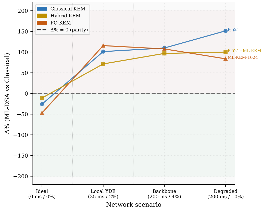
QUIC
