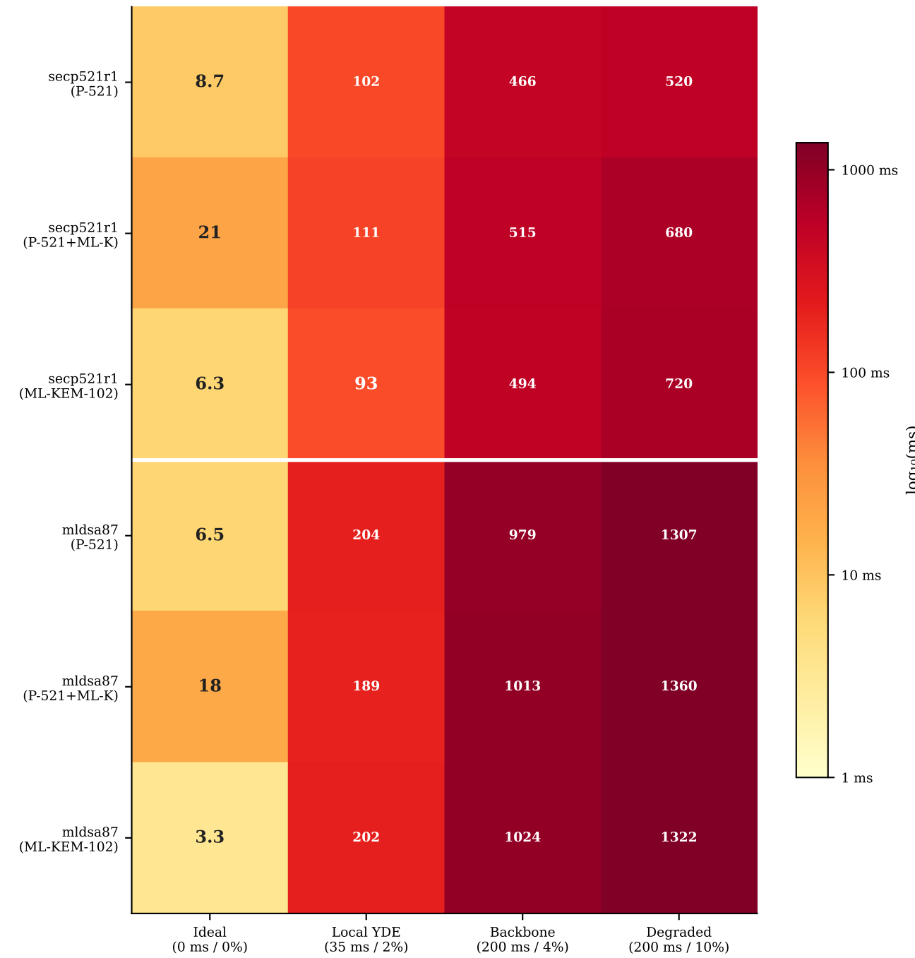
QUIC
